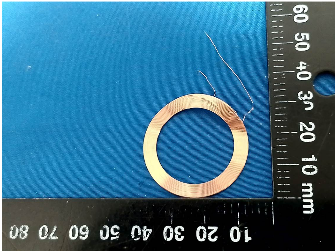
Loop Antenna(125kHz)
