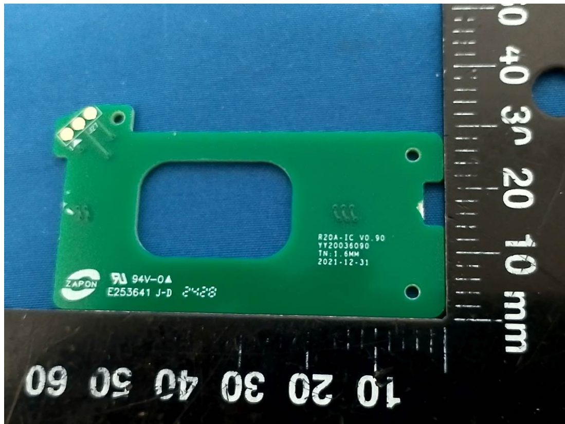
Loop Antenna(13.56MHz)
