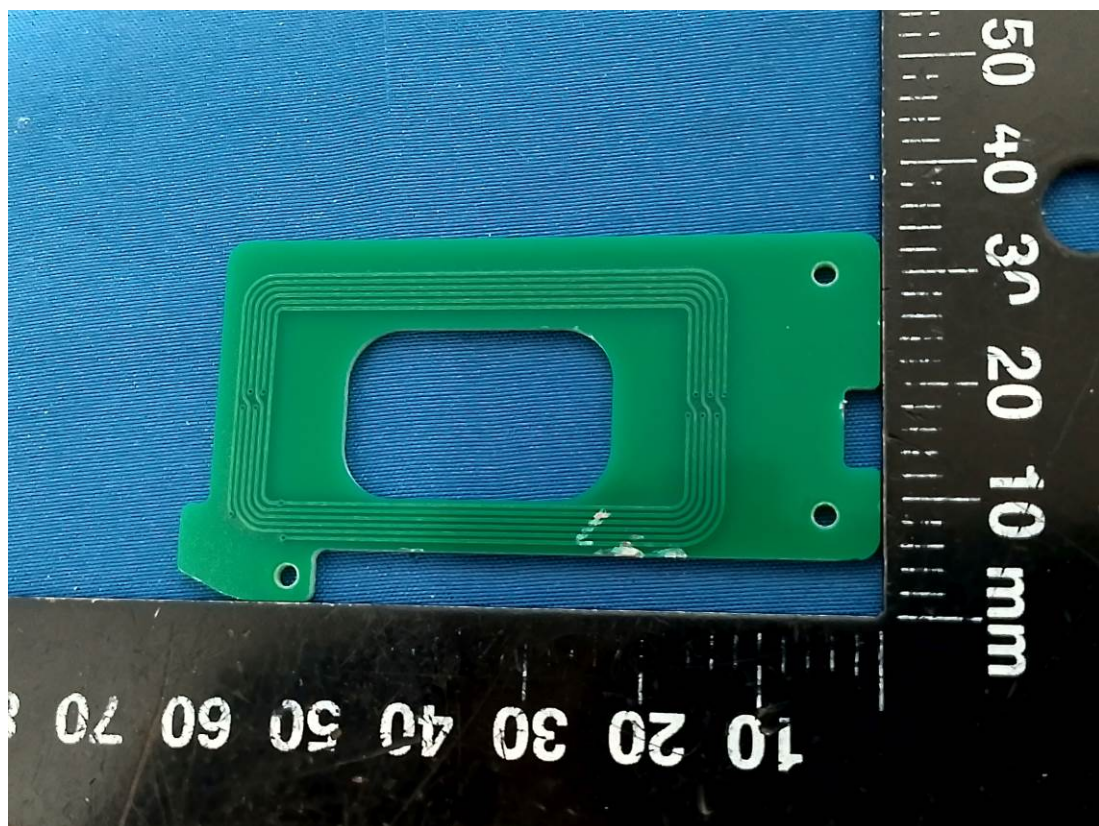
Loop Antenna(13.56MHz)
