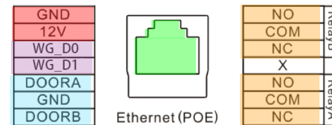
Figure 1.2-1 Connector Interface
