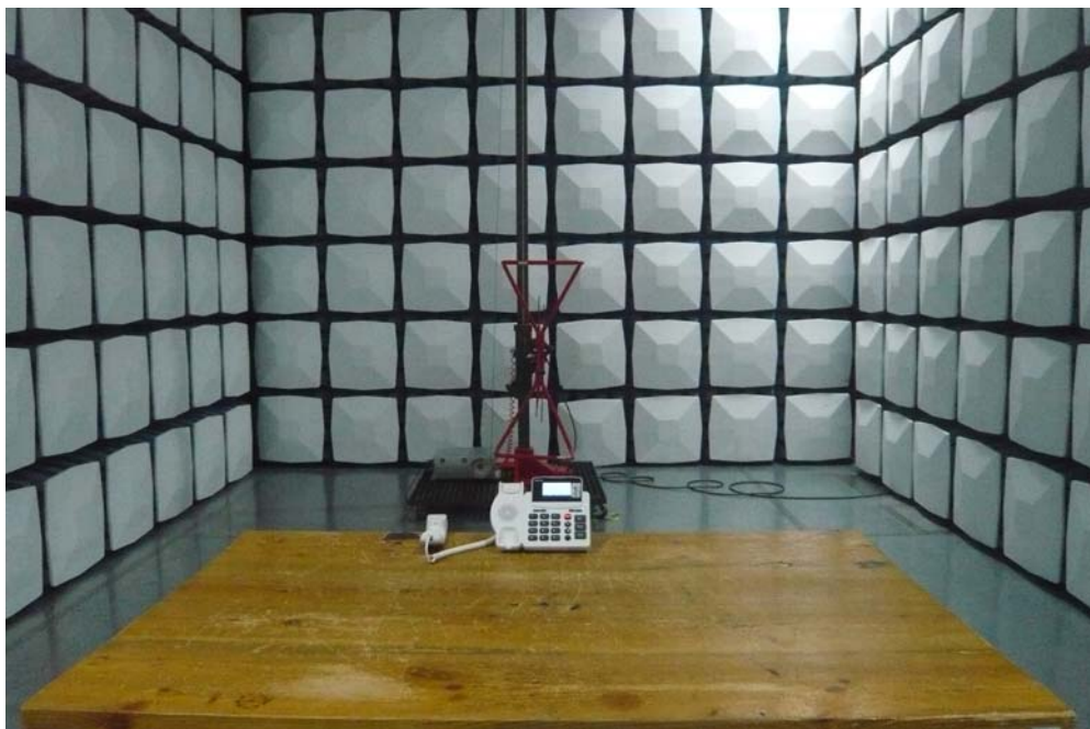
Radiated Emission –Front View (POE)
