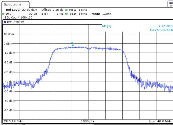
a_5180MHz_Chain 0
