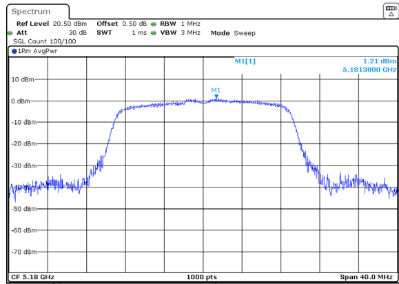
ac20_5180MHz_Chain 0
