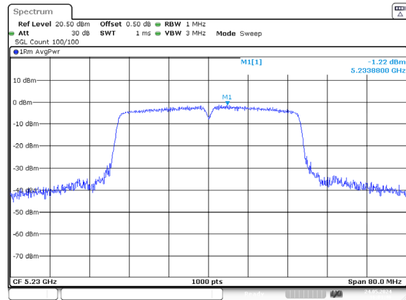
ac40_5230MHz_Chain 0
