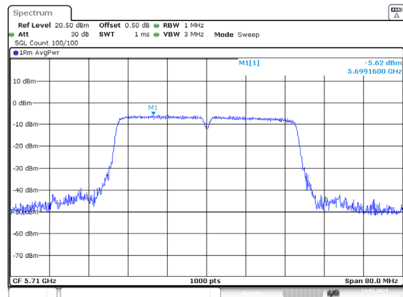
ac40_5710MHz_Chain 0
