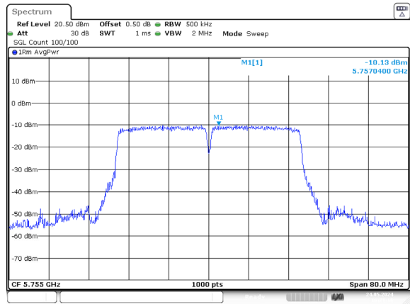
ac40_5755MHz_Chain 0
