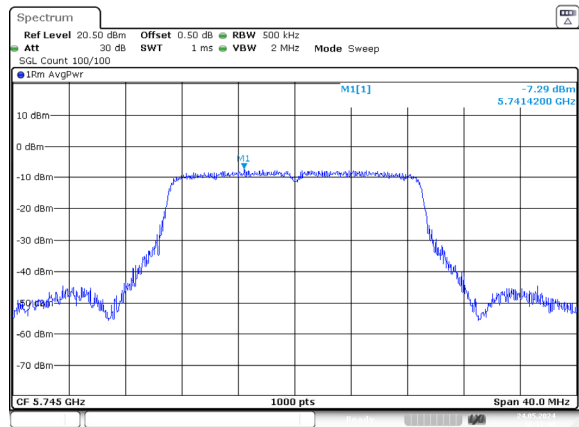
ac20_5745MHz_Chain 0
