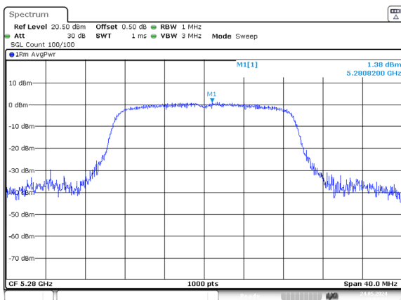
ac20_5280MHz_Chain 0
