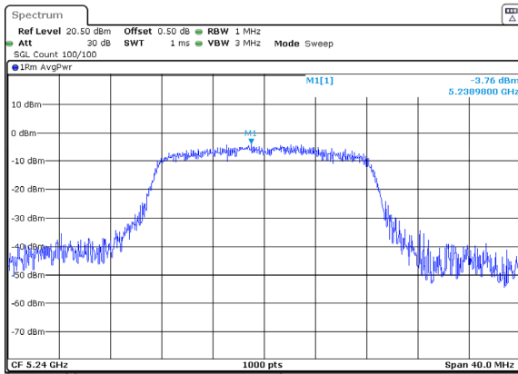
a_5240MHz_Chain 0
