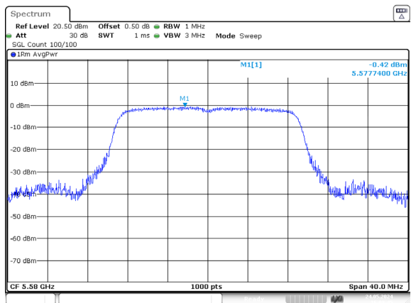
ac20_5580MHz_Chain 0
