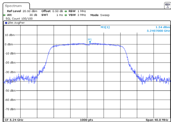
ac20_5240MHz_Chain 0
