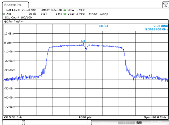
ac40_5310MHz_Chain 0
