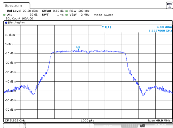
ac20_5825MHz_Chain 0
