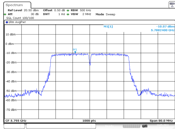
ac40_5795MHz_Chain 0
