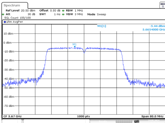
ac40_5670MHz_Chain 0
