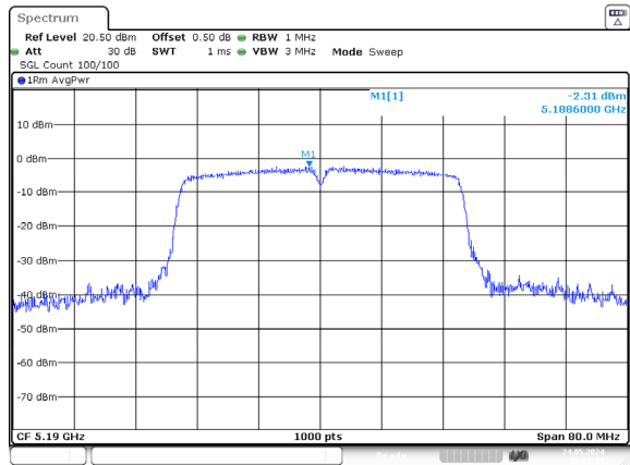
ac40_5190MHz_Chain 0
