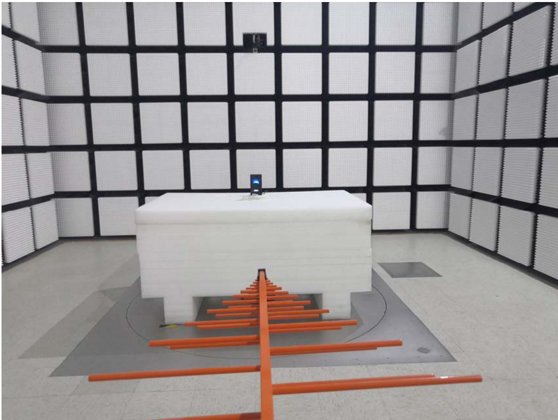
Radiated Emission Below 1GHz Adapter- A05C
