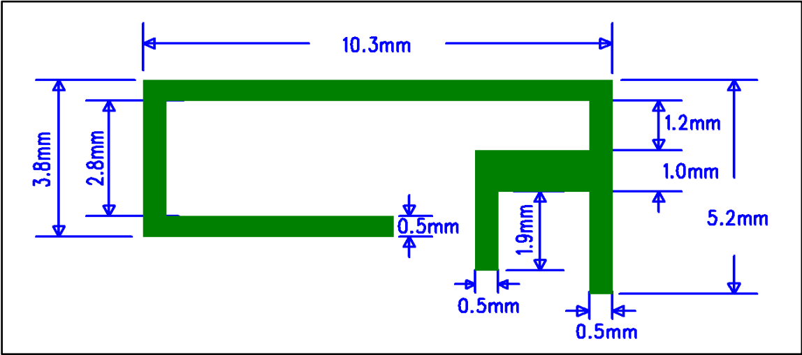
Antenna Dimension
