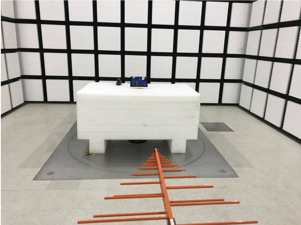
Radiated Emissions Below1G rear View -POE
