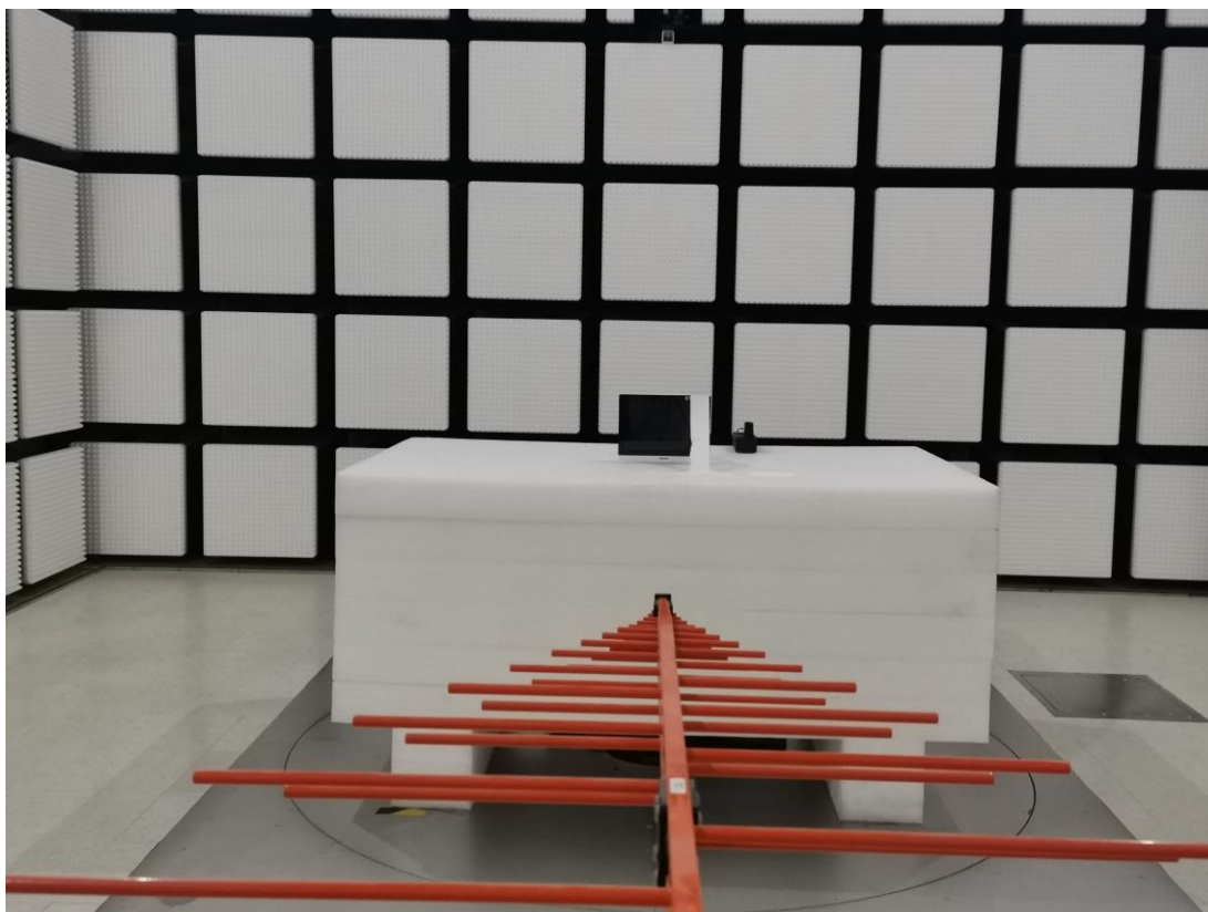
Radiated Emission Below 1GHz View-Adapter Mode
