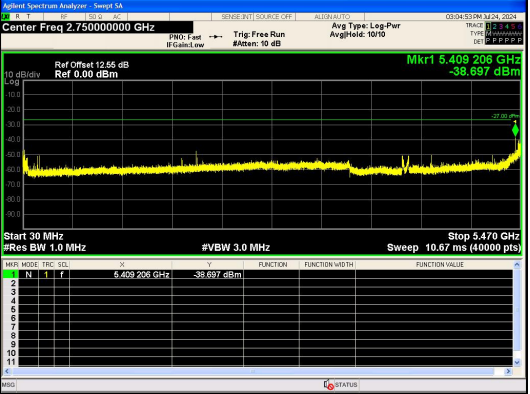
Spurious Emission:30.0~5470 MHz IEEE 802.11ac_Channel 122_80MHz_Antenna 0
