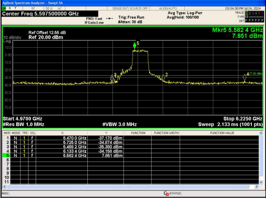
Out Of Band Emission IEEE 802.11ac_Channel 122_80MHz_Antenna 0
