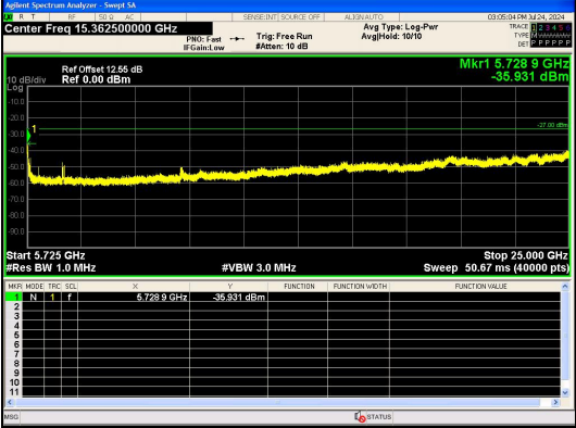
Spurious Emission:5725~25000.0 MHz IEEE 802.11ac_Channel 122_80MHz_Antenna 0
