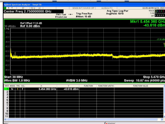
Spurious Emission:30.0~5470 MHz IEEE 802.11n Channel 102 40MHz Antenna (
