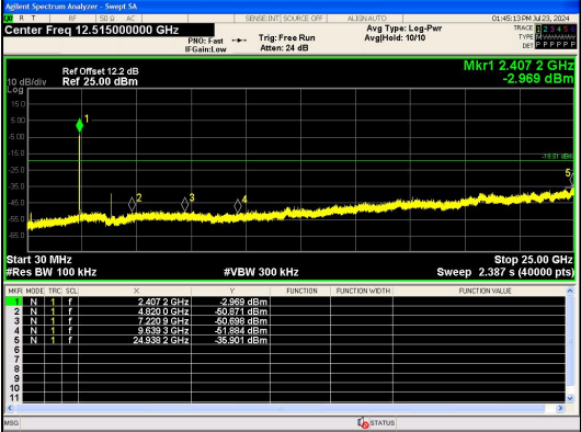
Spurious Emission IEEE 802.11n_Channel 1_20MHz_Antenna 0
