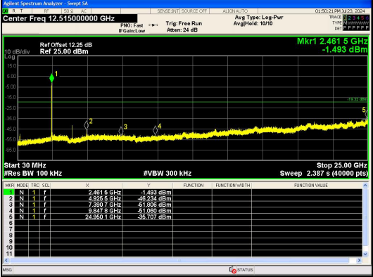
Spurious Emission IEEE 802.11n_Channel 11_20MHz_Antenna 0
