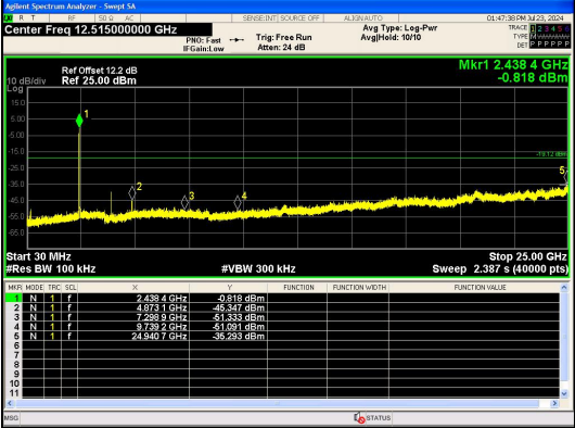
Spurious Emissions IEEE 802.11n_Channel 6_20MHz_Antenna 0
