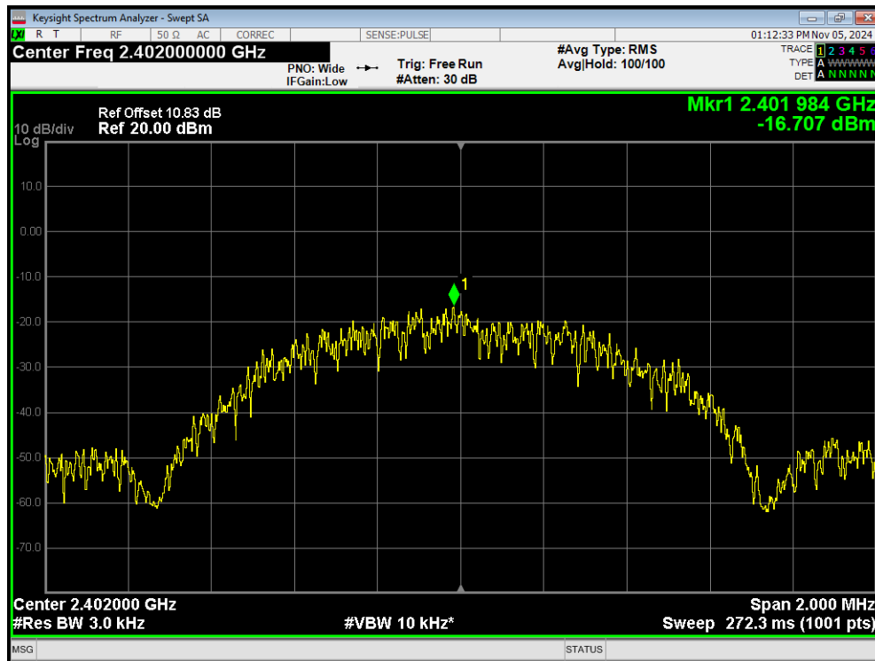
PSD Bluetooth LE (1M) 2402MHz
