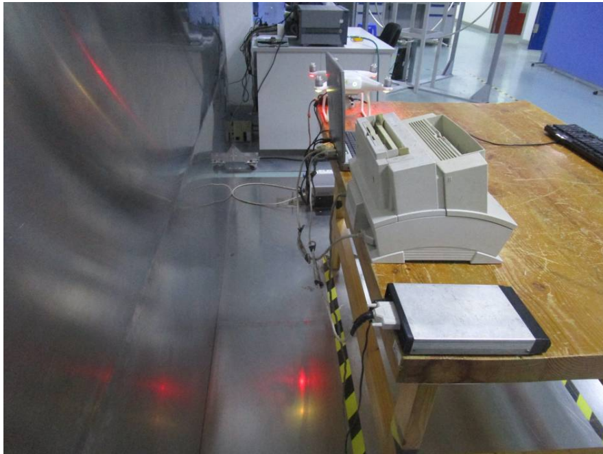
Conducted Emission – Side View (Downloading Mode)
