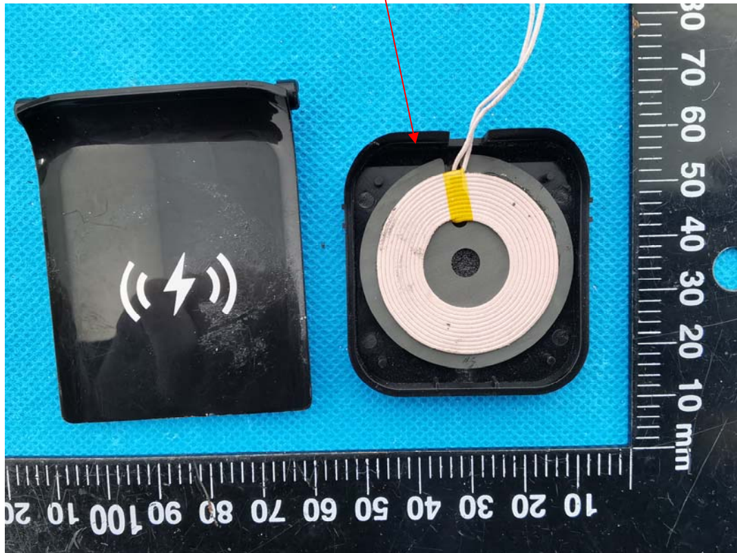
Airpods Coil
