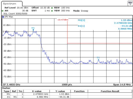
3DH1_Hopping_Upper
