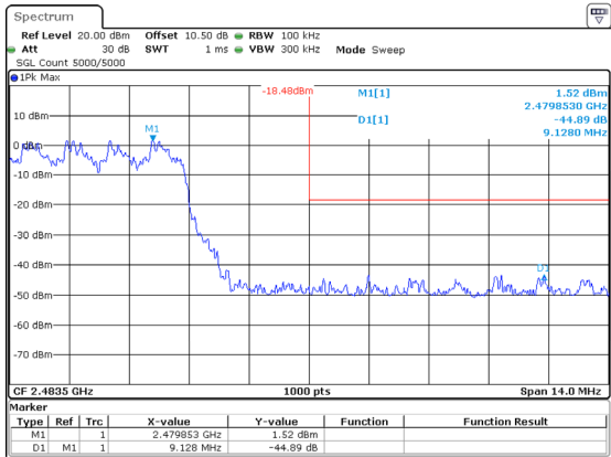
2DH1_Hopping_Upper
