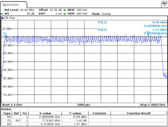
3DH1_Hopping 79
