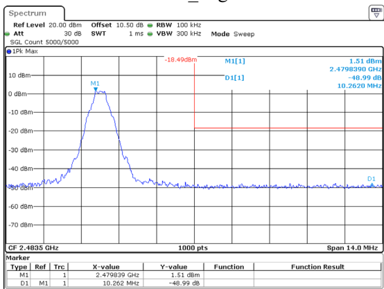
DH1_High
