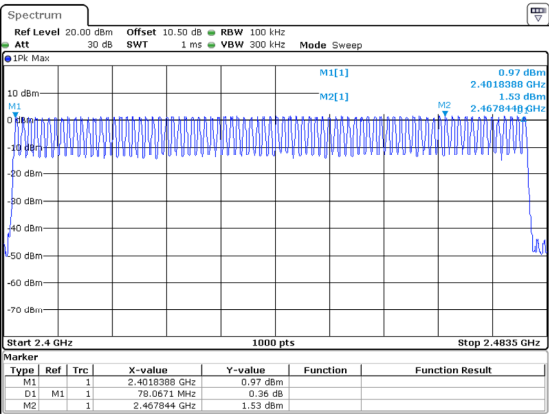
DH1_Hopping 79
