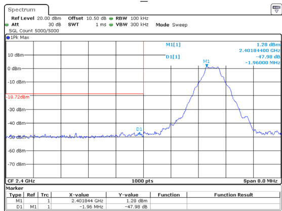
DH1_Low
