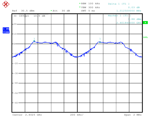
DH1_Low 1.013MHz
