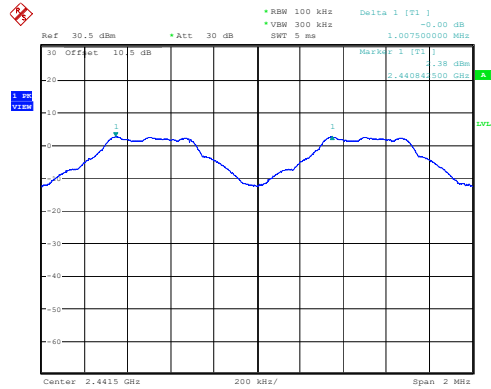
DH1_Middle 1.007MHz
