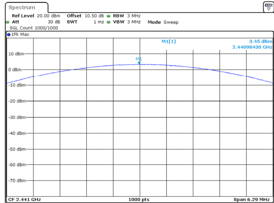
3DH1_Middle 3.45dBm
