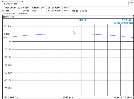
DH1_Low 0.29dBm
