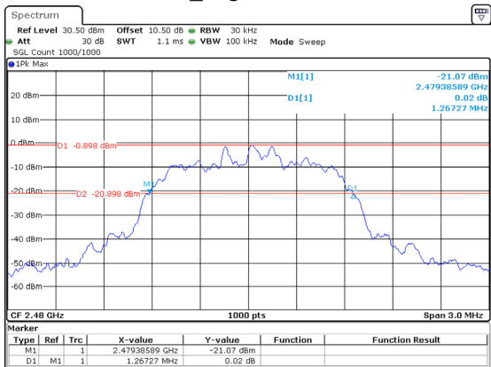
2DH1_High 1.267MHz
