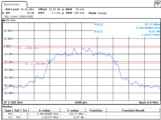
2DH1_Low 1.267MHz
