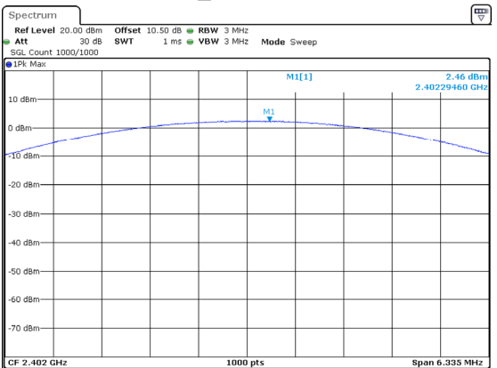
2DH1_Low 2.46dBm
