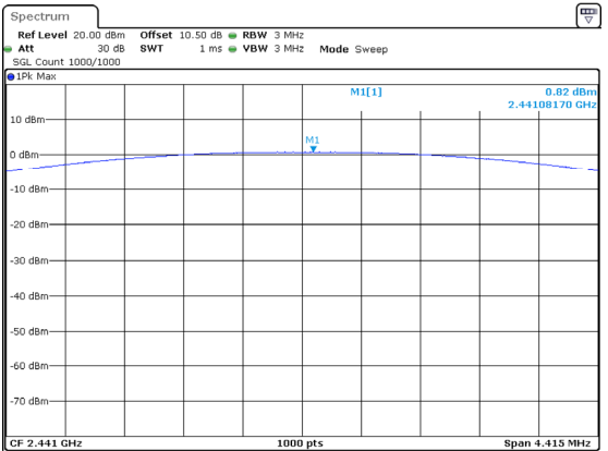
DH1_Middle 0.82dBm
