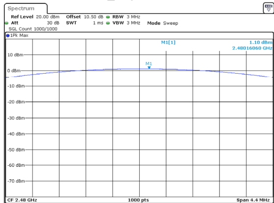
DH1_High 1.10dBm
