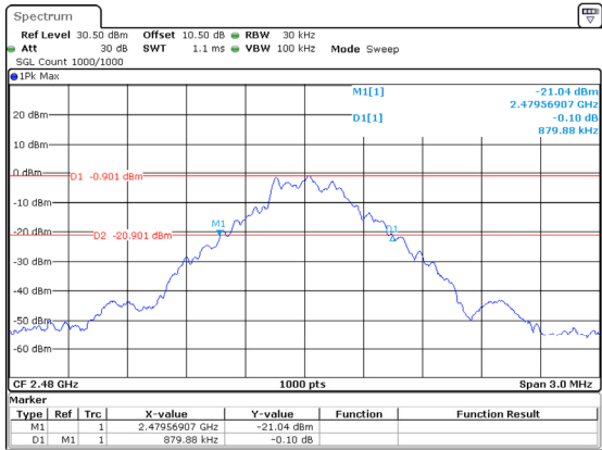
DH1_High 0.880MHz
