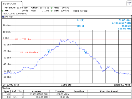
DH1_Low 0.856MHz
