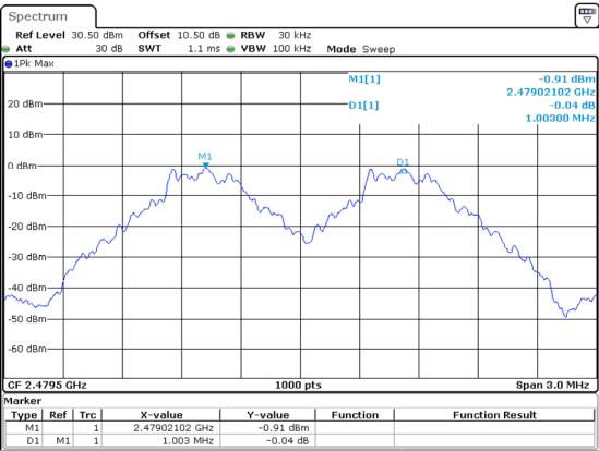
DH1_High 1.003MHz
