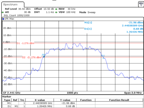
2DH1_Middle 1.264MHz
