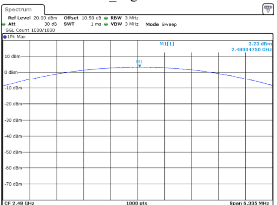
2DH1_High 3.23dBm
