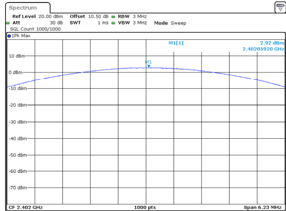
3DH1_Low 2.92dBm
