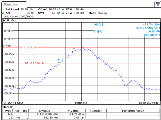
DH1_Middle 0.883MHz
