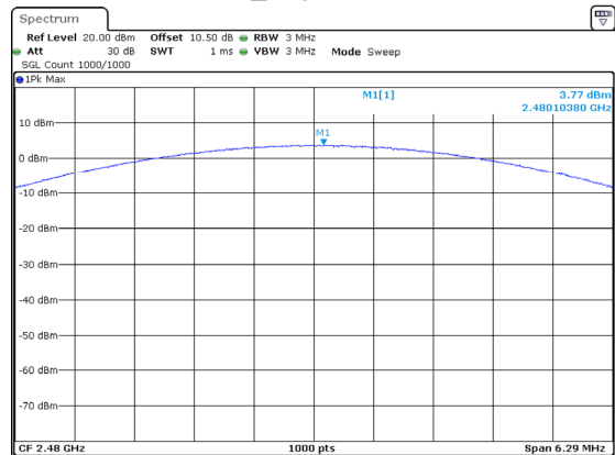
3DH1_High 3.77dBm
