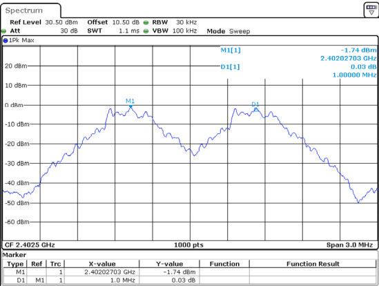
DH1_Low 1MHz
