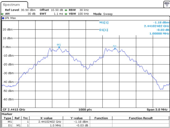
DH1_Middle 1MHz
