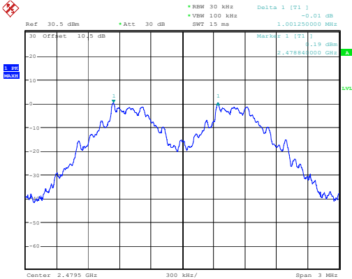
GFSK_High 1.001MHz
