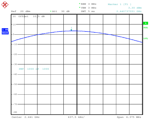
8DPSK_Middle 3.30dBm
