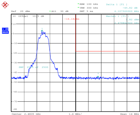
8DPSK_High
