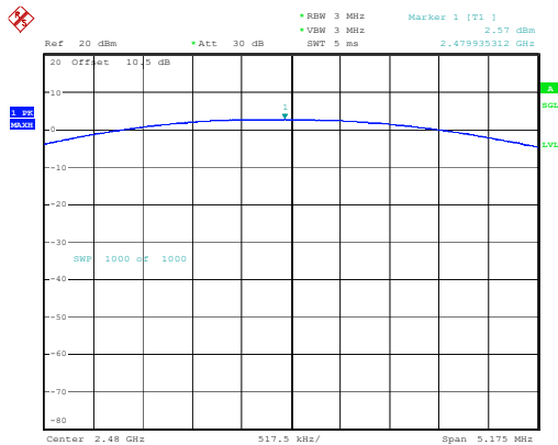
GFSK_High 2.57dBm
