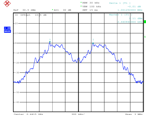
GFSK_Middle 1.001MHz
