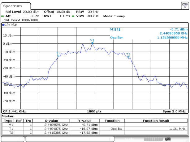
3DH1_Middle
