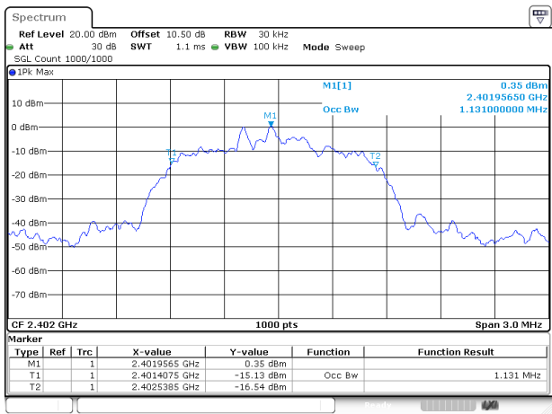
3DH1_Low
