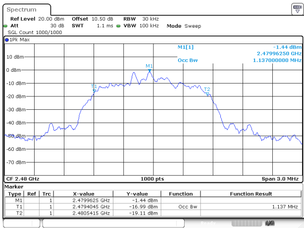
3DH1_High
