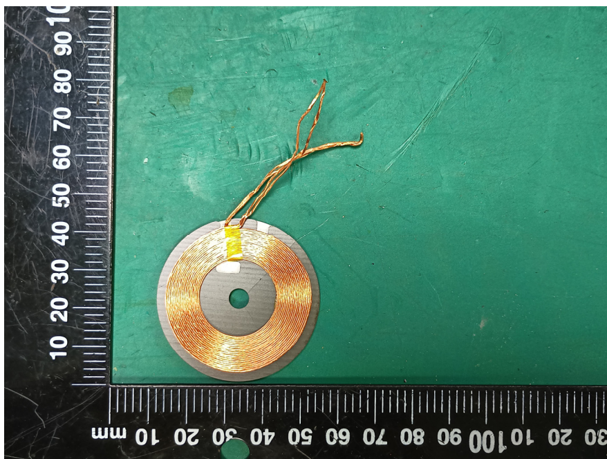
Coil Antenna
