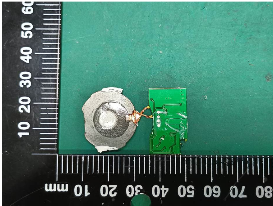
Coil for Watch
