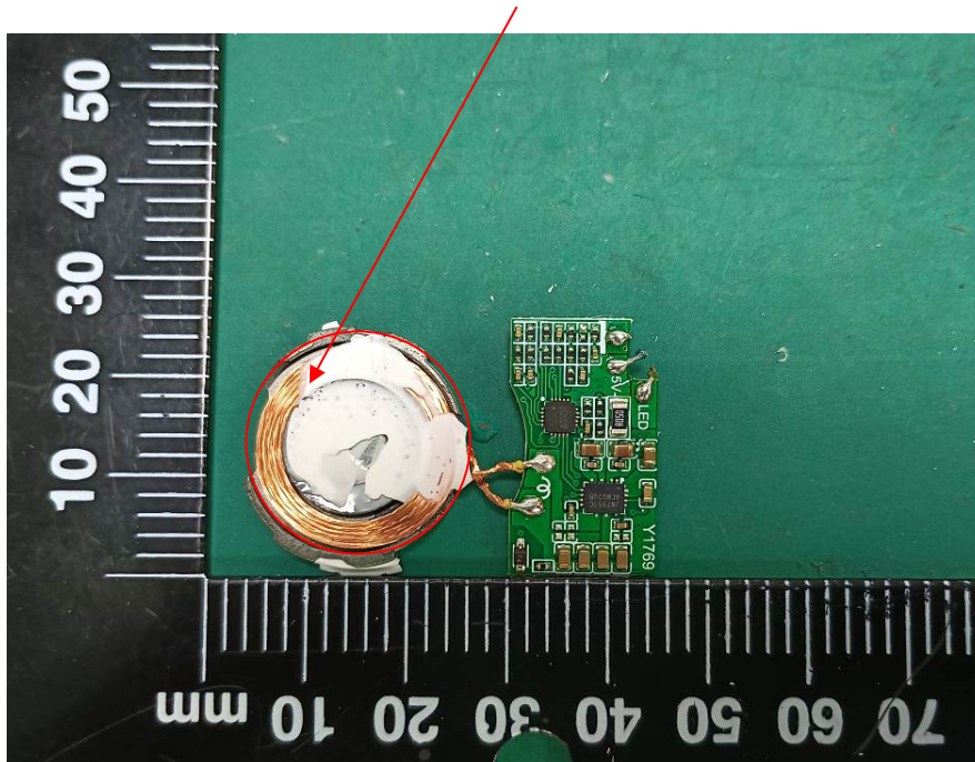
Coil for Watch
