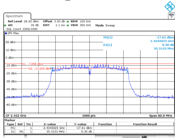
802.11n40_2452MHz 35.315MHz
