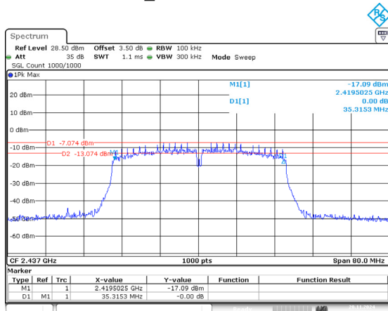
802.11n40_2437MHz 35.315MHz
