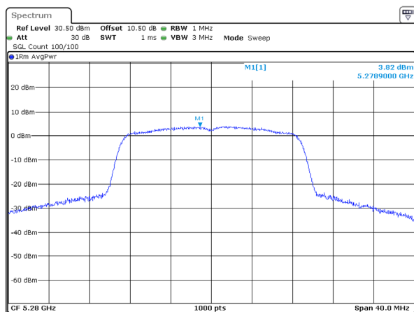
802.11n20_5280MHz
