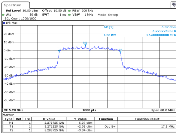
802.11n20_5280MHz
