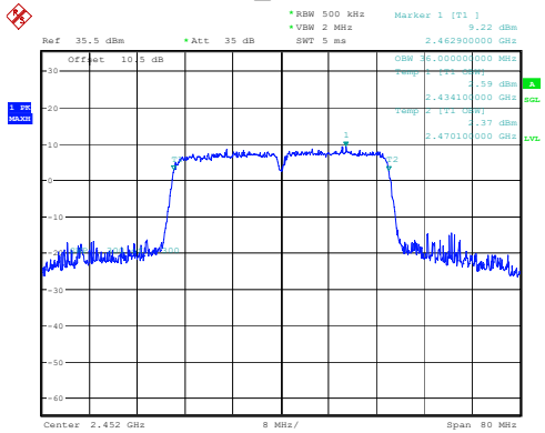
802.11n40_2452MHz 36MHz
