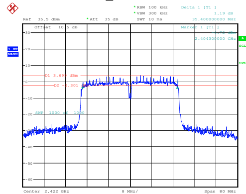
802.11n40_2422MHz 35.400MHz
