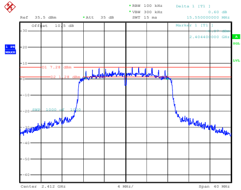
802.11n20_2412MHz 15.550MHz
