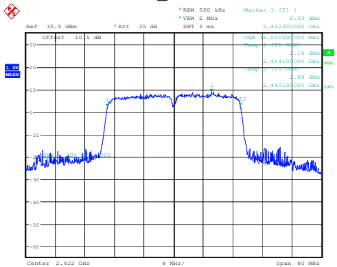
802.11n40_2422MHz 36MHz
