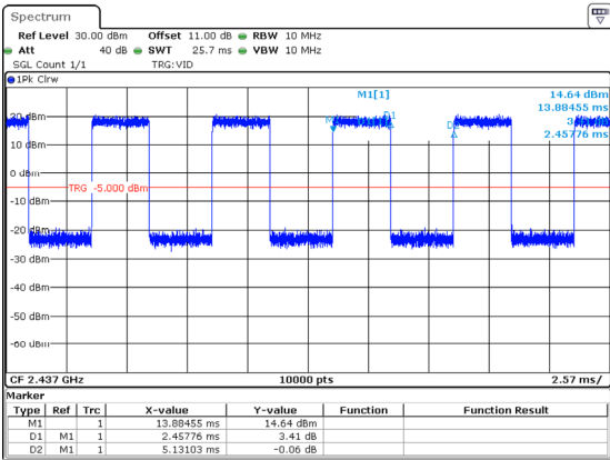
802.11n40_2437MHz
