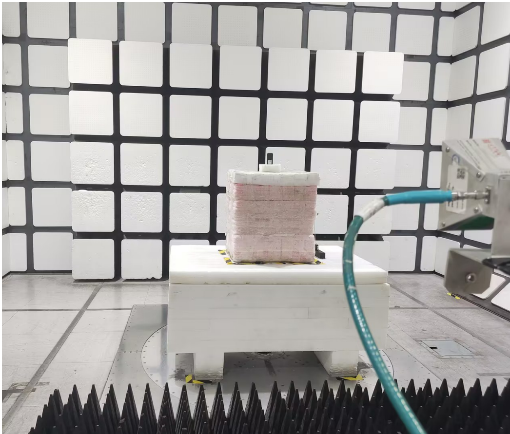
Radiated Emissions View (18-25 GHz)
