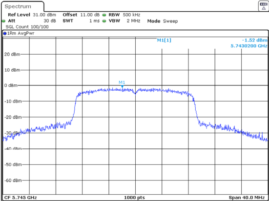
802.11n20_5745MHz
