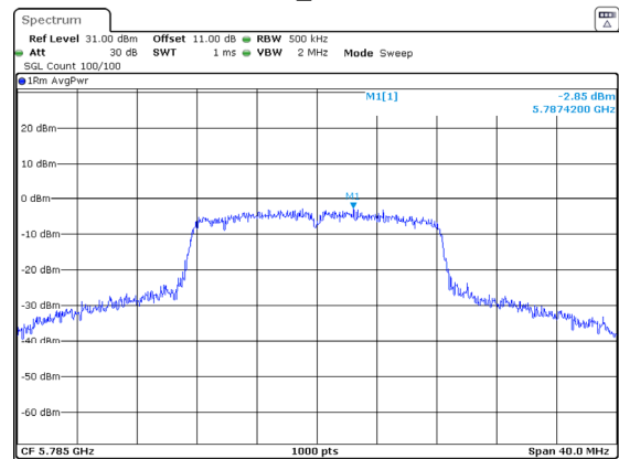
802.11a_5785MHz
