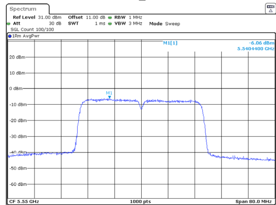
802.11n40_5550MHz
