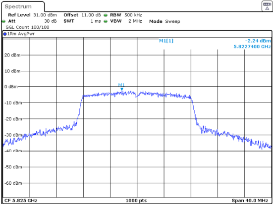
802.11a_5825MHz
