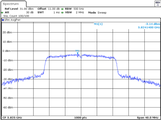
802.11n20_5825MHz
