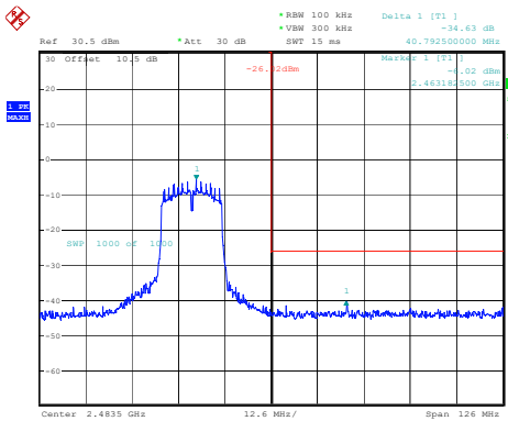
802.11g_2462MHz
