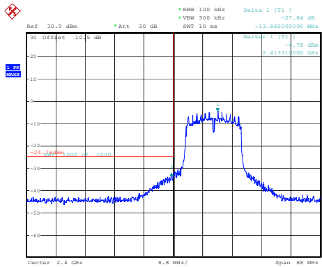
802.11g_2412MHz
