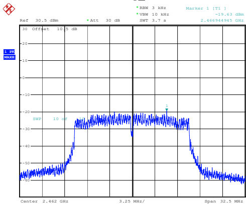
802.11g_2462MHz
