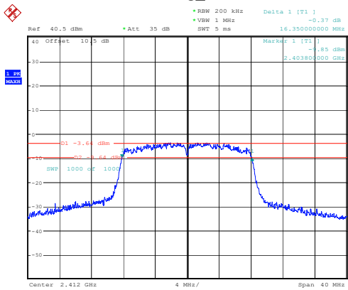
802.11g_2412MHz
