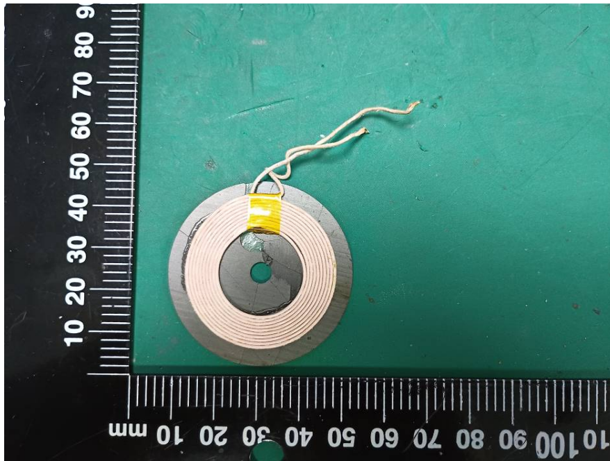
WPT Antenna
