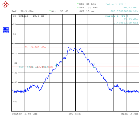
DH1_High 0.889MHz
