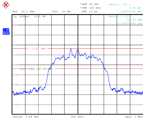
2DH1_High 1.256MHz
