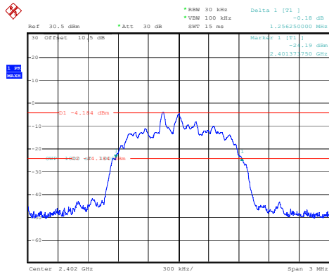
2DH1_Low 1.256MHz
