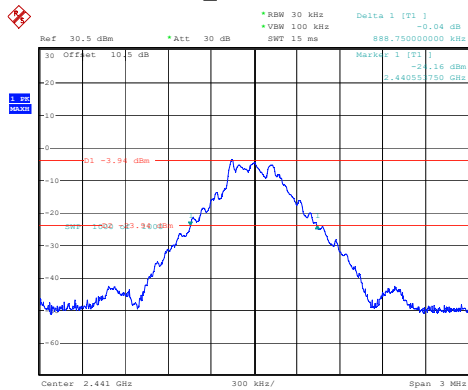
DH1_Middle 0.889MHz
