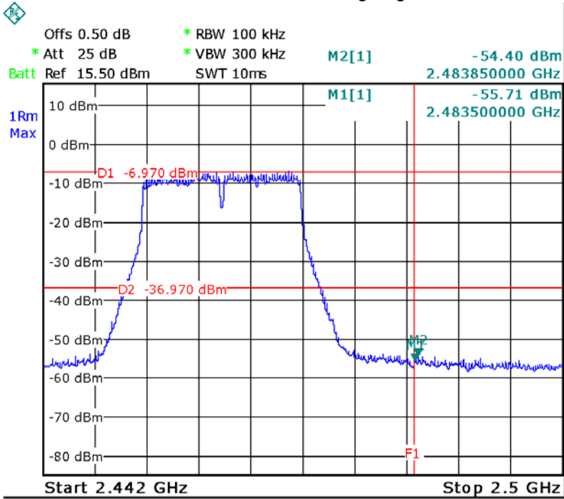
ANTA TX 11n HT20: Band edge-right side
