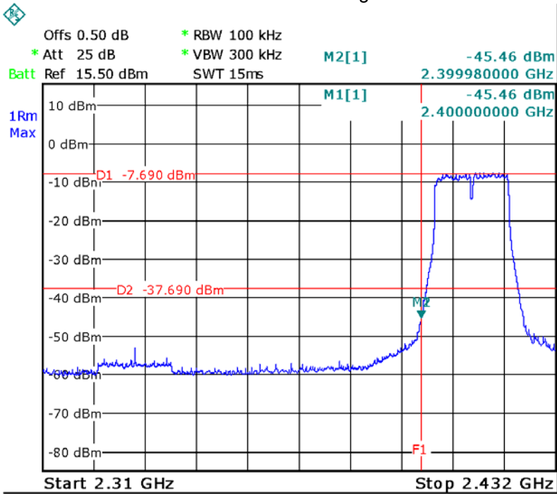
ANTA TX 11n HT20: Band edge-left side
