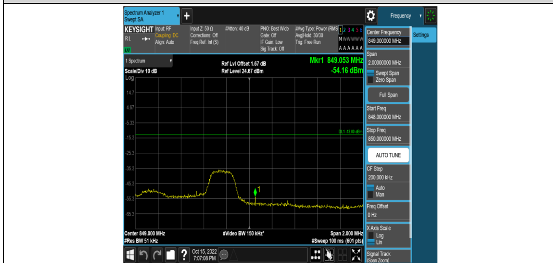
Band5-3MHz-16QAM-20635-1RB#14
