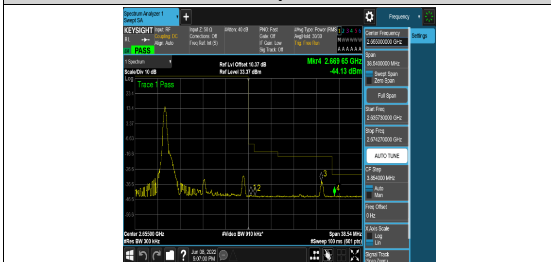
Band41-15MHz-16QAM-41165-1RB#0
