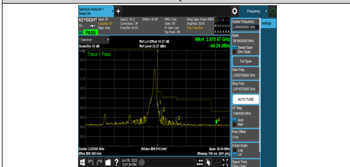
Band41-15MHz-16QAM-41165-1RB#74
