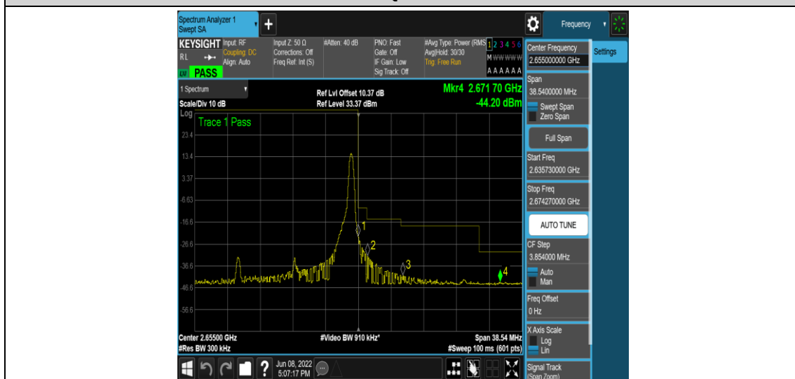
Band41-15MHz-QPSK-41165-1RB#74
