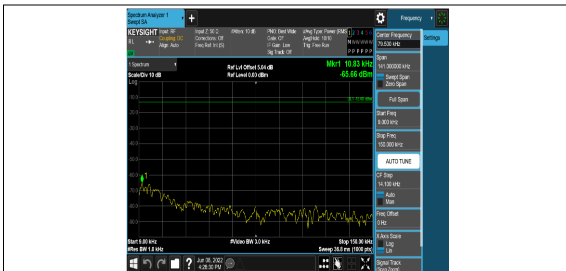
Band41-5MHz-QPSK-40740-1RB#0-Range1:0.009~0.15MHz
