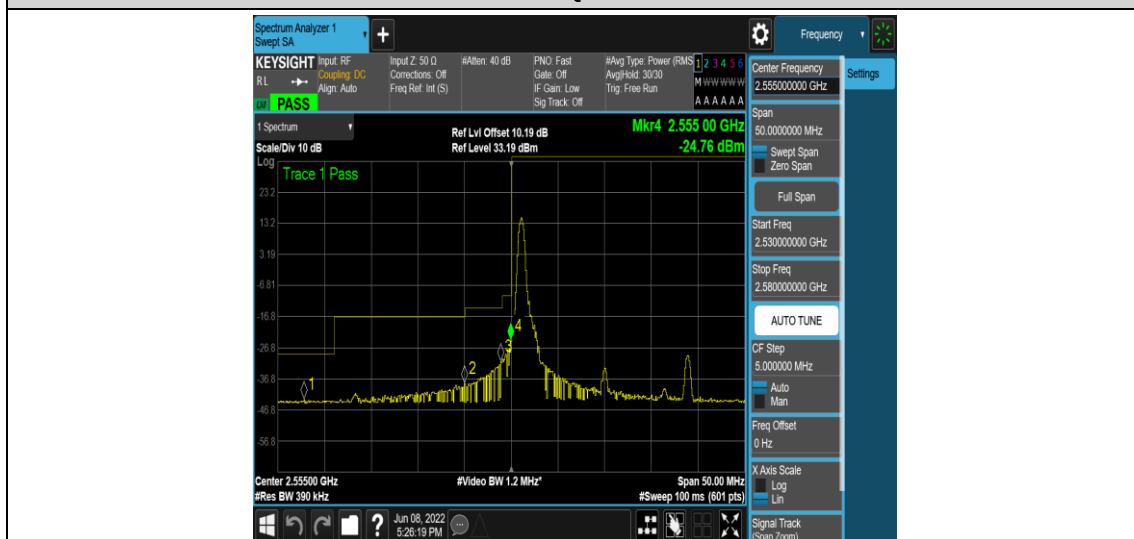
Band41-20MHz-QPSK-40340-1RB#0
