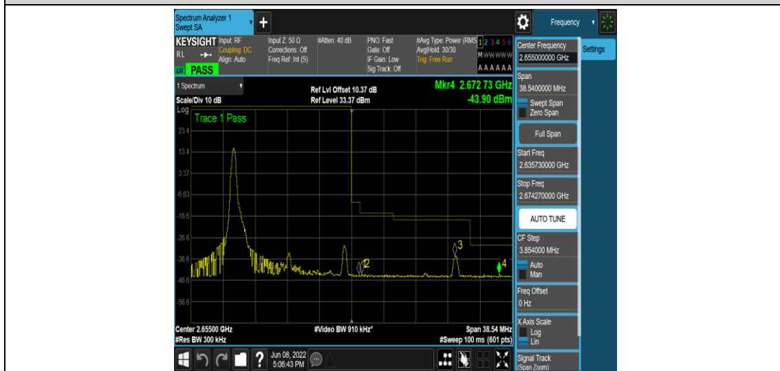
Band41-15MHz-QPSK-41165-1RB#0
