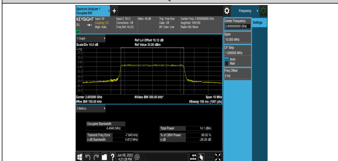
Band41-5MHz-16QAM-40740-25RB#0
