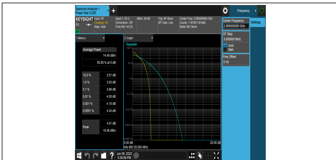
Band41-20MHz-QPSK-40340-1RB#0
