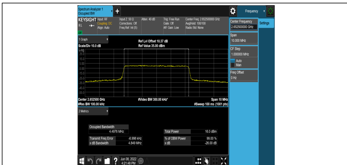
Band41-5MHz-QPSK-41215-25RB#0
