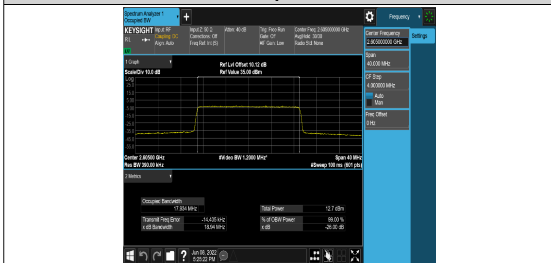
Band41-20MHz-16QAM-40740-100RB#0
