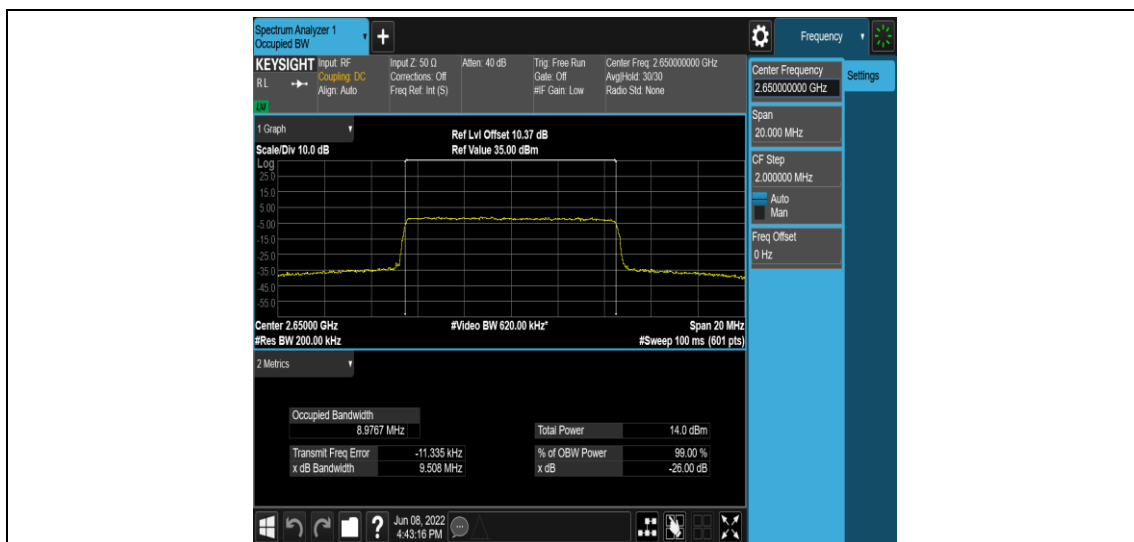
Band41-10MHz-16QAM-41190-50RB#0
