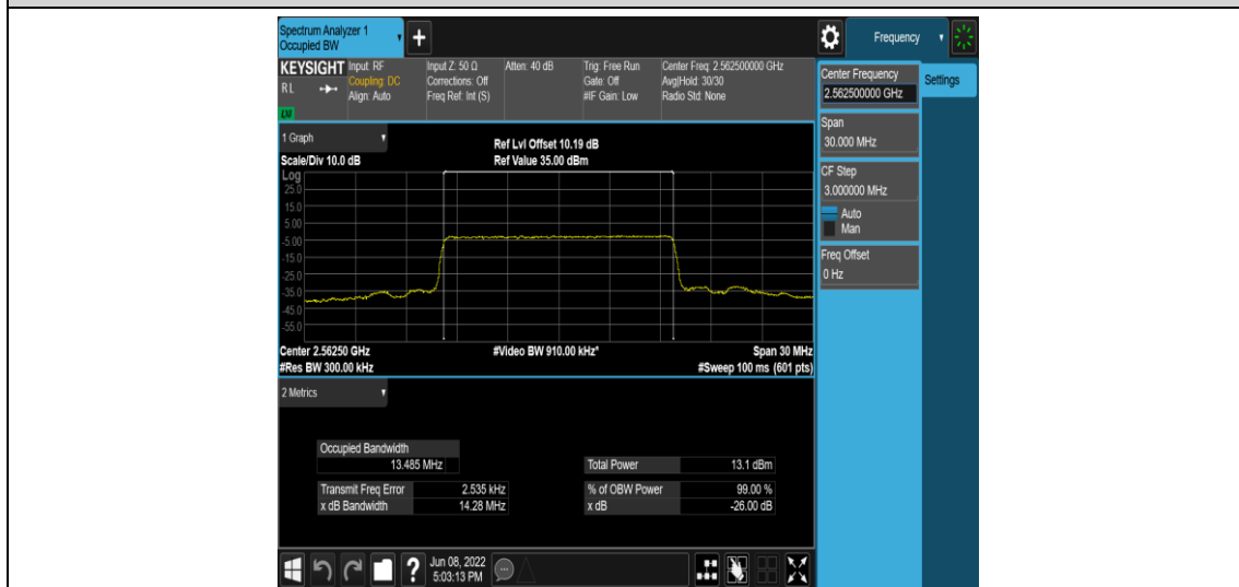
Band41-15MHz-QPSK-40315-75RB#0
