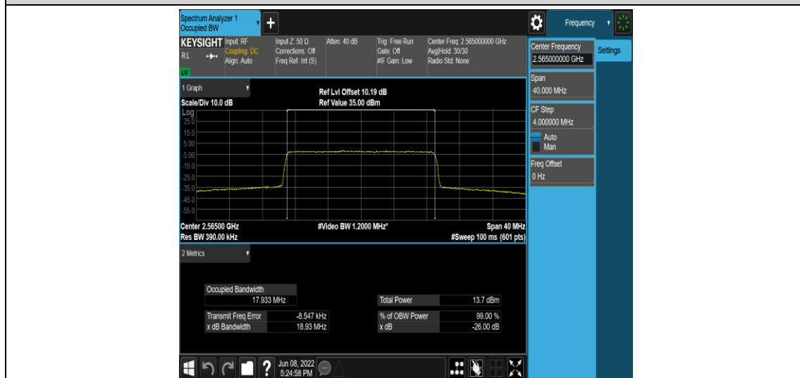
Band41-20MHz-16QAM-40340-100RB#0
