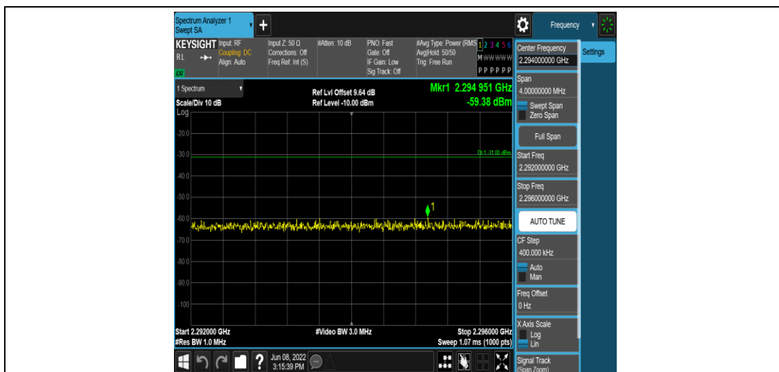
Band40-5MHz-QPSK-39200-1RB#0-Range6:2292~2296MHz
