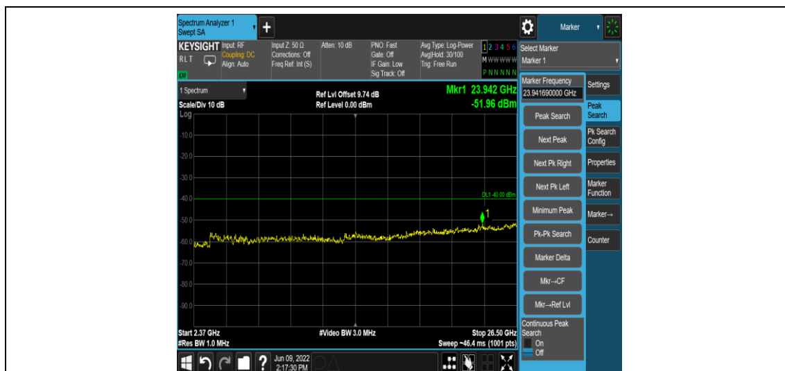
Band40-5MHz-16QAM-39200-1RB#0-Range15:2365~26500MHz
