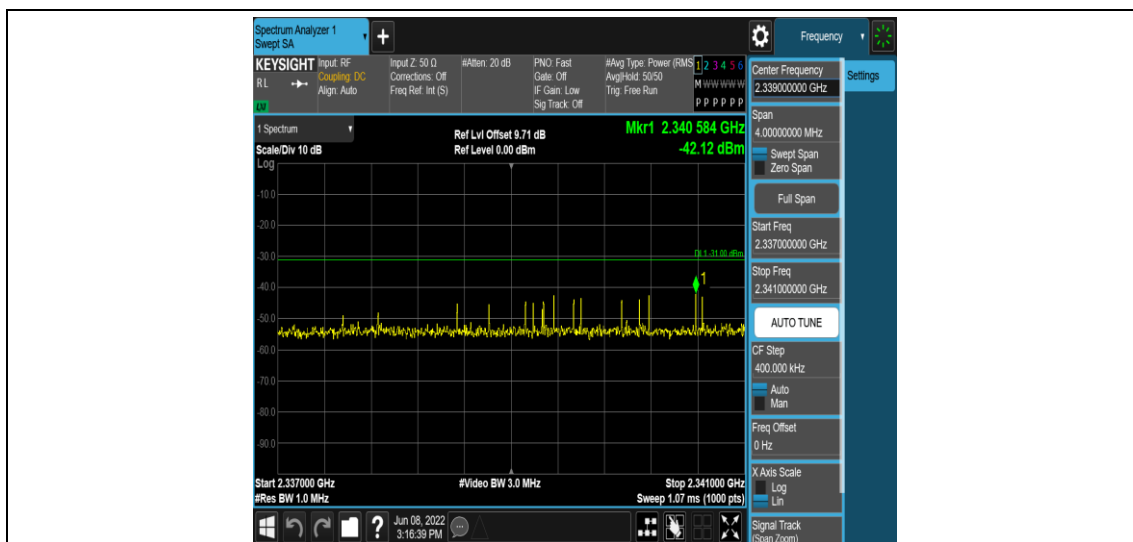
Band40-5MHz-QPSK-39200-1RB#0-Range12:2337~2341MHz
