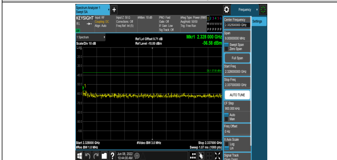
Band40-5MHz-QPSK-38775-1RB#0-Range11:2328~2337MHz
