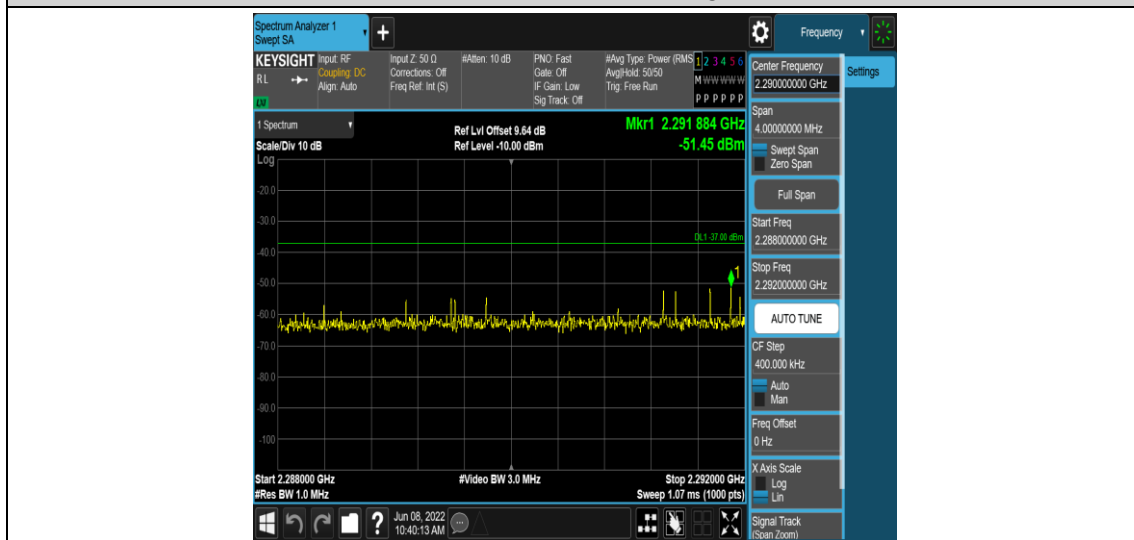
Band40-5MHz-16QAM-38750-1RB#0-Range5:2288~2292MHz
