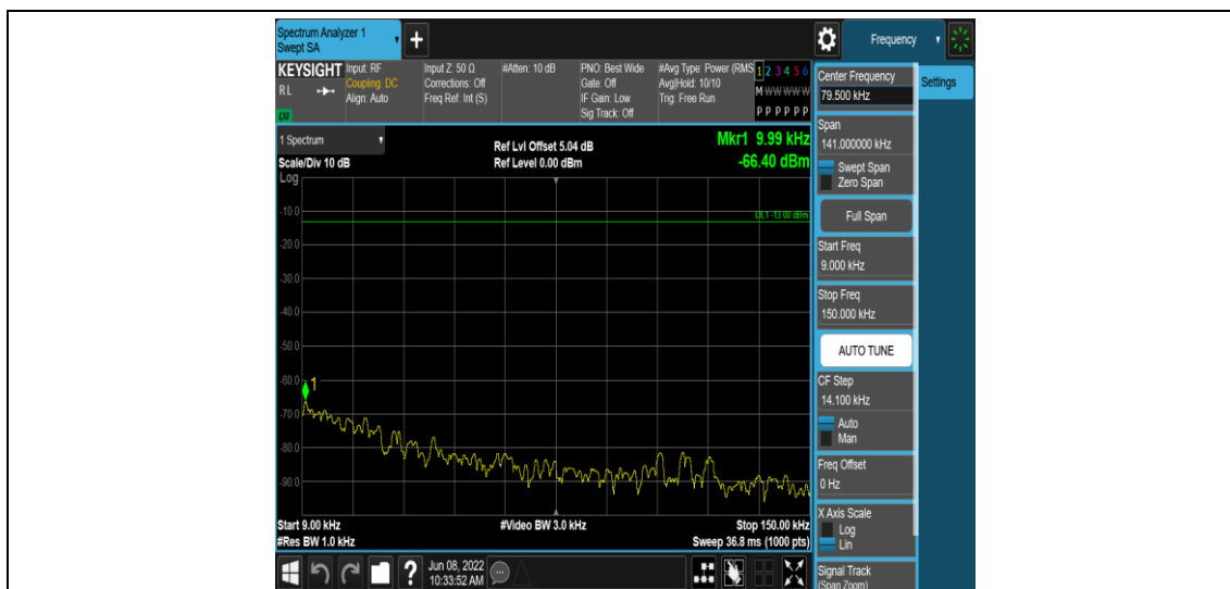
Band40-5MHz-16QAM-38725-1RB#0-Range1:0.009~0.15MHz
