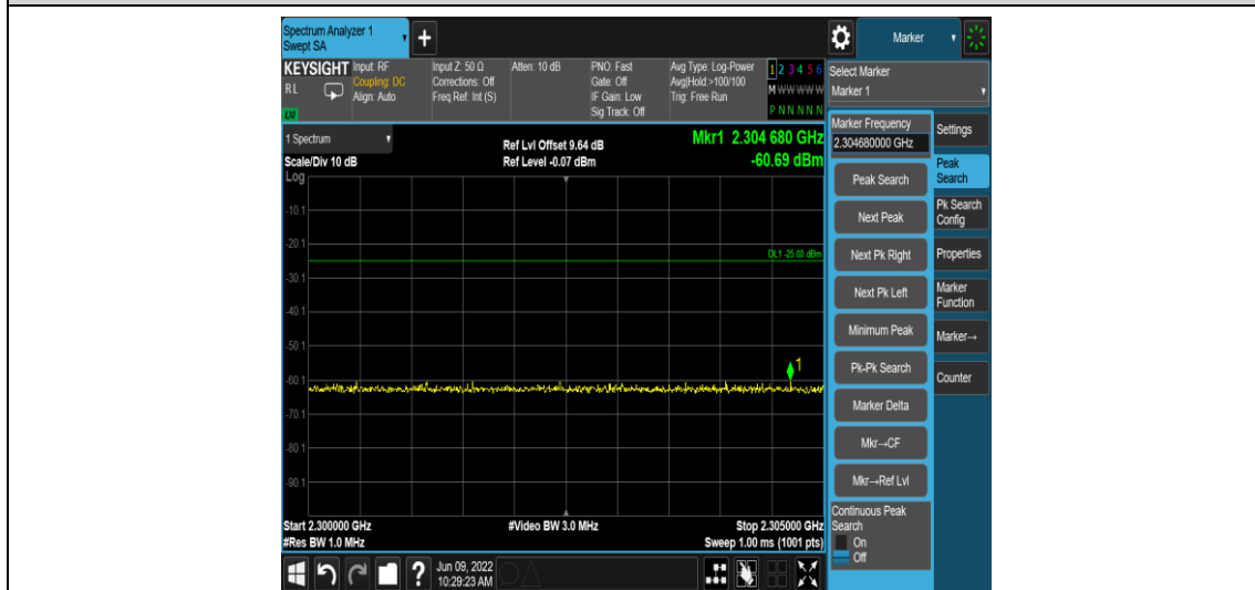
Band40-5MHz-16QAM-38750-1RB#0-Range8:2300~2305MHz
