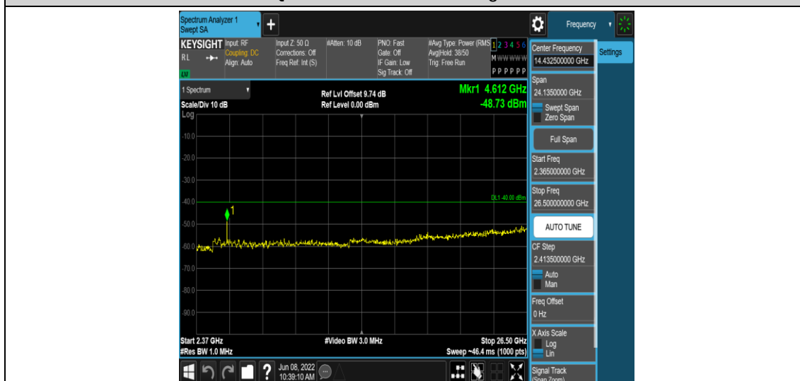
Band40-5MHz-QPSK-38750-1RB#0-Range15:2365~26500MHz
