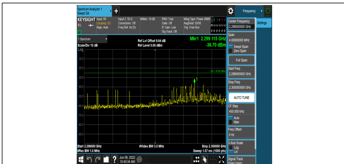
Band40-5MHz-16QAM-38750-1RB#0-Range7:2296~2300MHz
