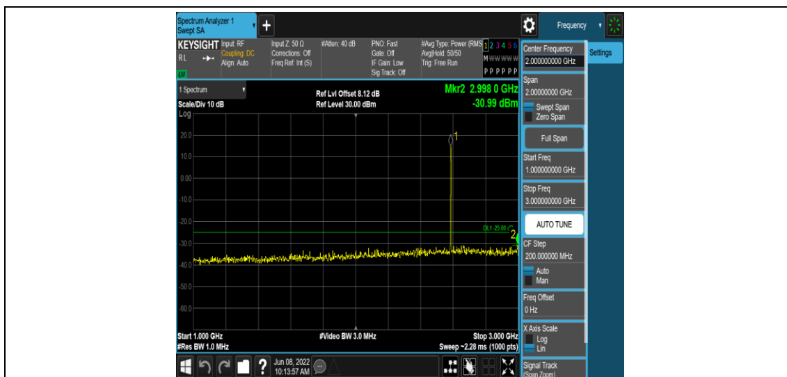
Band38-20MHz-16QAM-38000-1RB#0-Range4:1000~3000MHz
