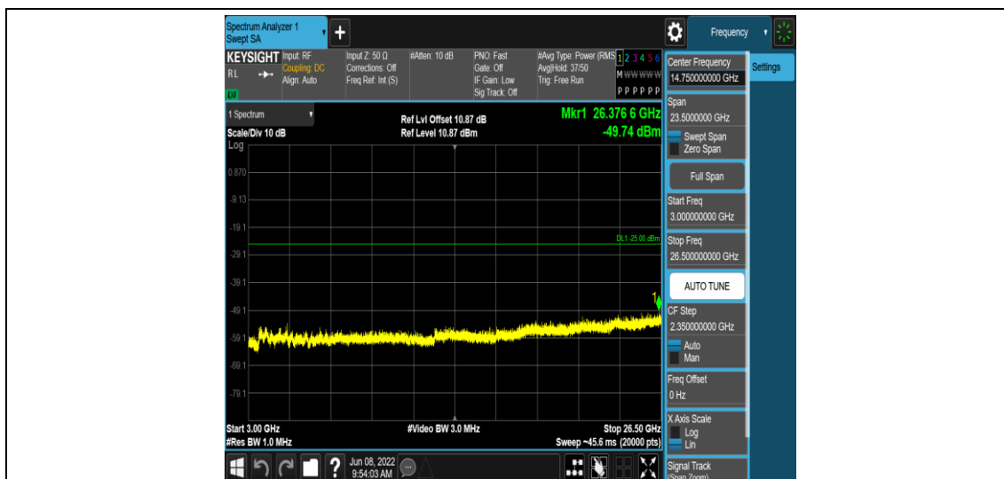
Band38-15MHz-QPSK-38175-1RB#0-Range5:3000~26500MHz
