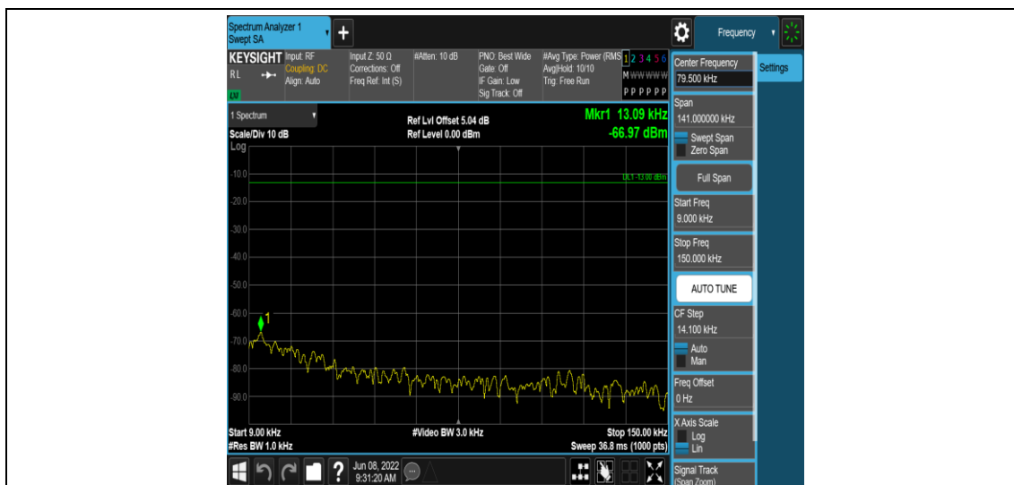
Band38-10MHz-16QAM-38000-1RB#0-Range1:0.009~0.15MHz
