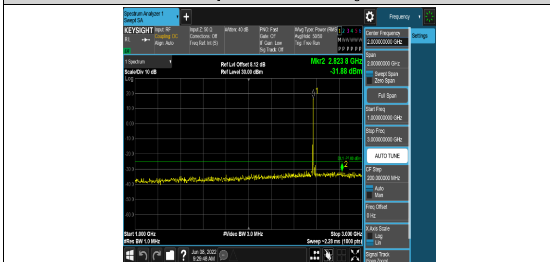
Band38-10MHz-16QAM-37800-1RB#0-Range4:1000~3000MHz
