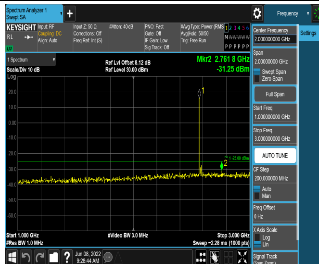
Band38-10MHz-QPSK-37800-1RB#0-Range4:1000~3000MHz
