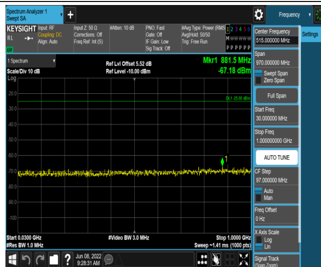
Band38-10MHz-QPSK-37800-1RB#0-Range3:30~1000MHz
