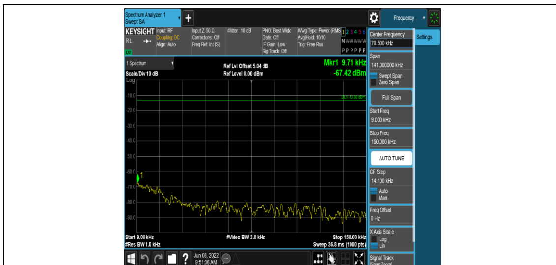
Band38-15MHz-QPSK-38000-1RB#0-Range1:0.009~0.15MHz
