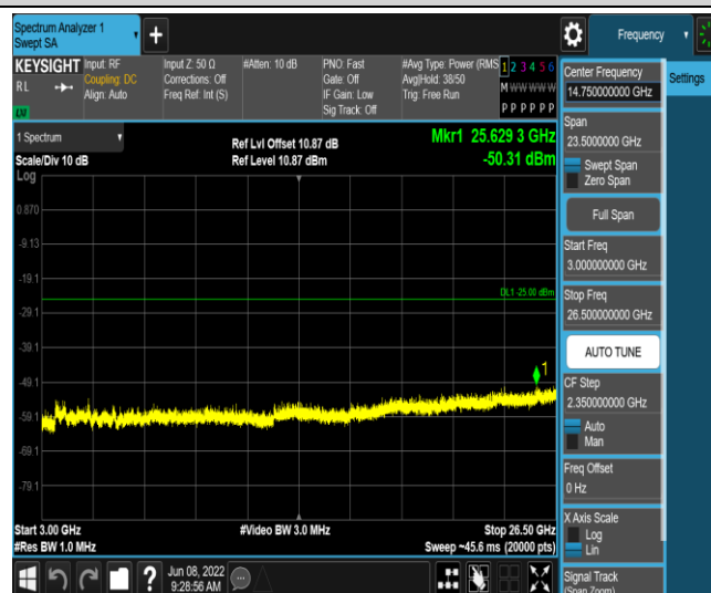
Band38-10MHz-QPSK-37800-1RB#0-Range5:3000~26500MHz
