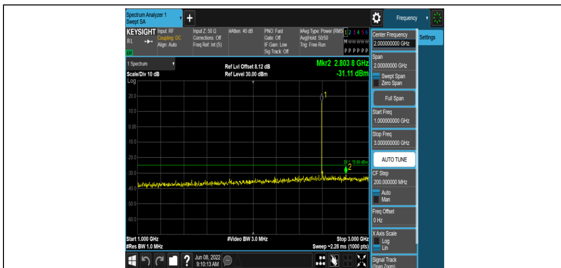
Band38-5MHz-QPSK-38000-1RB#0-Range4:1000~3000MHz
