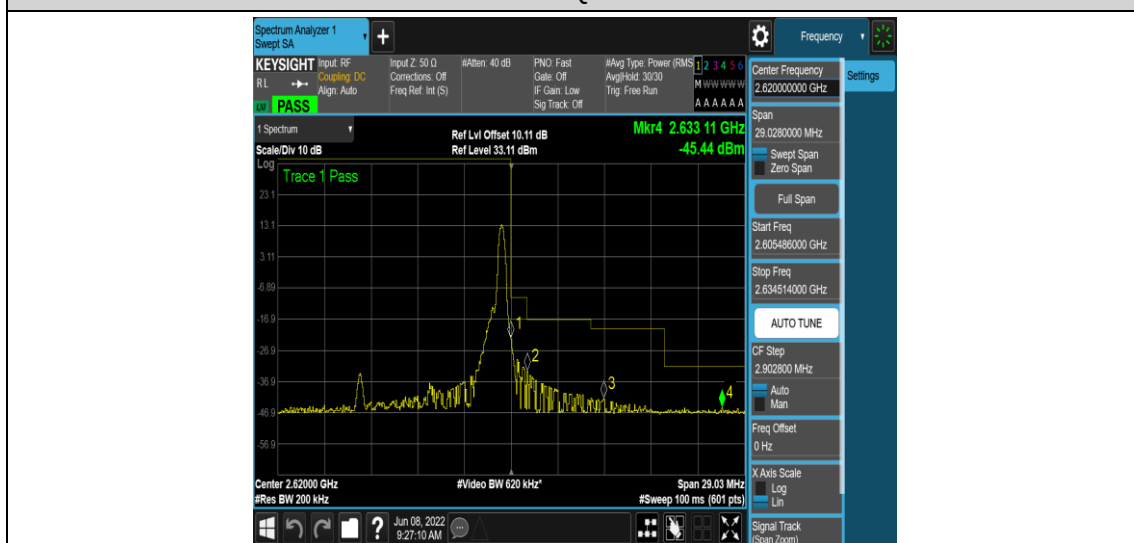
Band38-10MHz-16QAM-38200-1RB#49
