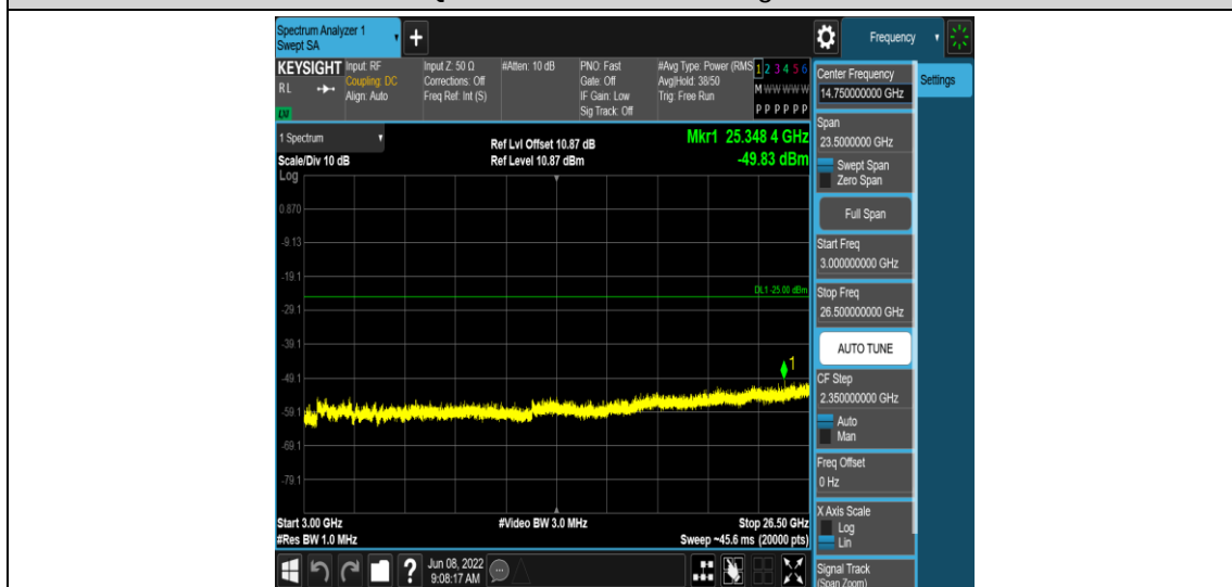
Band38-5MHz-QPSK-37775-1RB#0-Range5:3000~26500MHz
