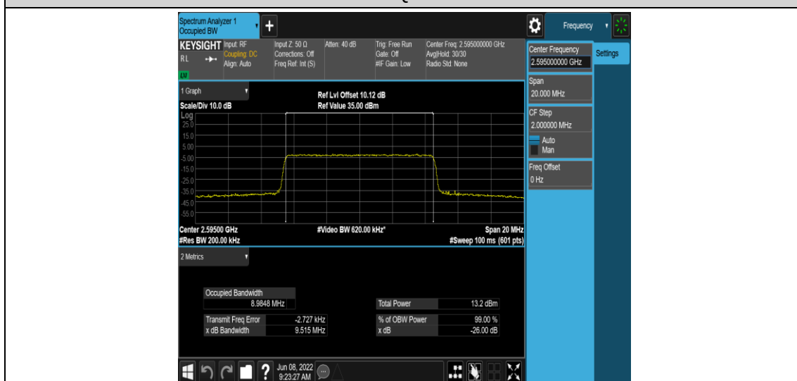
Band38-10MHz-16QAM-38000-50RB#0
