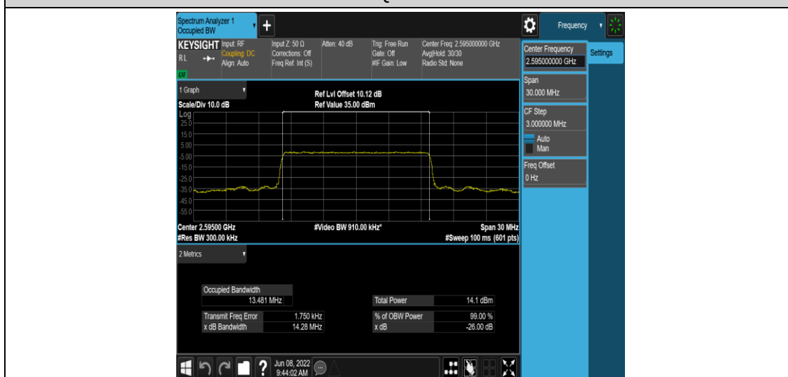
Band38-15MHz-QPSK-38000-75RB#0
