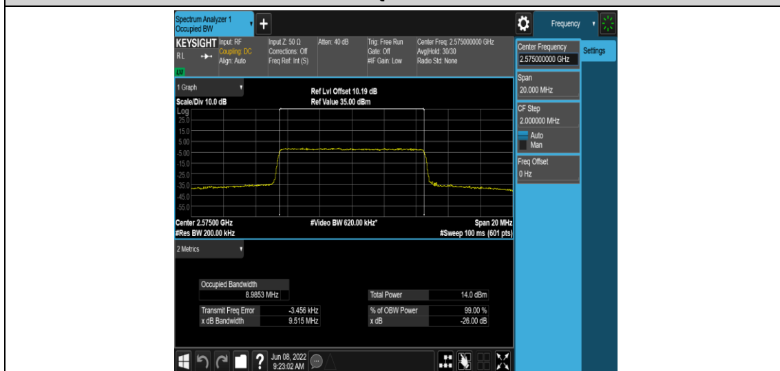
Band38-10MHz-16QAM-37800-50RB#0
