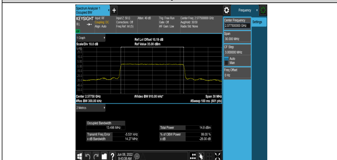
Band38-15MHz-QPSK-37825-75RB#0
