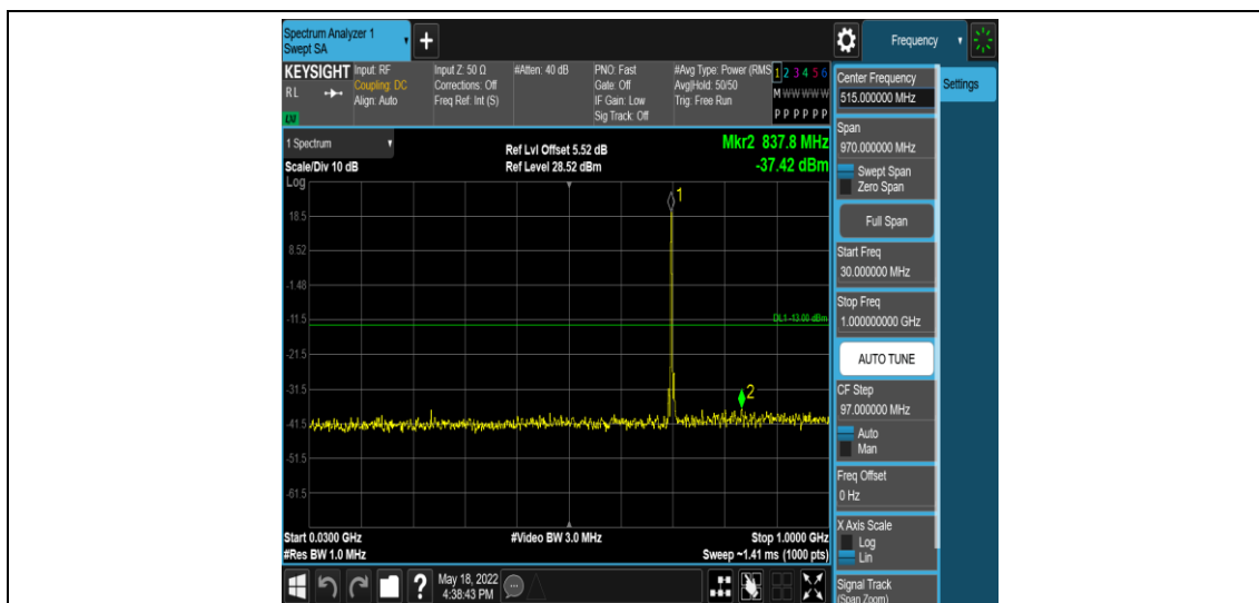
Band12-3MHz-QPSK-23095-1RB#0-Range3:30~1000MHz
