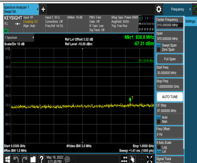
Band7-10MHz-QPSK-21100-1RB#0-Range3:30~1000MHz
