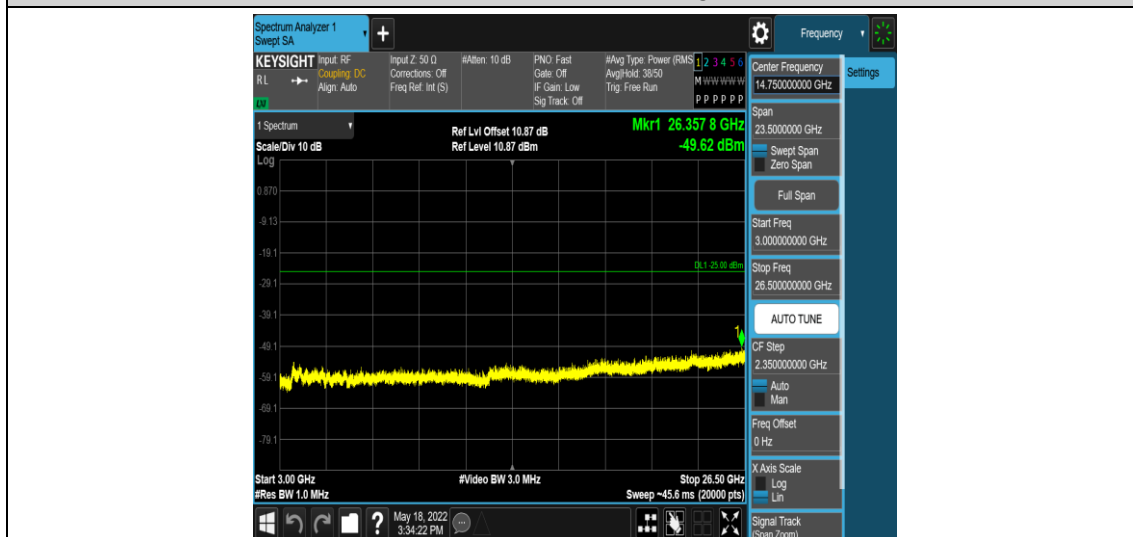
Band7-15MHz-QPSK-21100-1RB#0-Range5:3000~26500MHz
