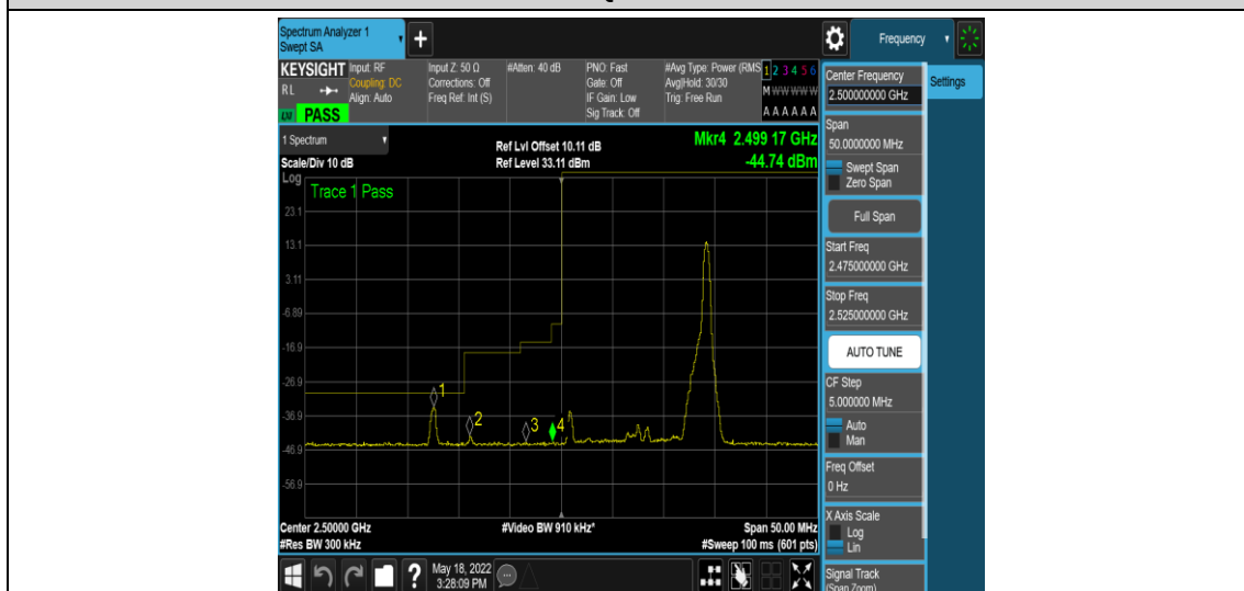
Band7-15MHz-QPSK-20825-1RB#74
