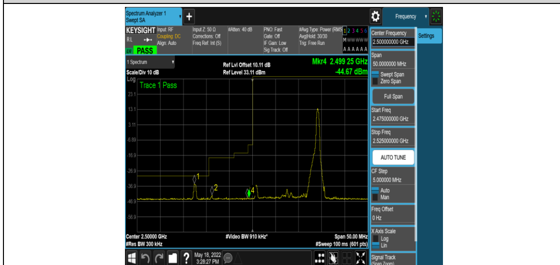
Band7-15MHz-16QAM-20825-1RB#74
