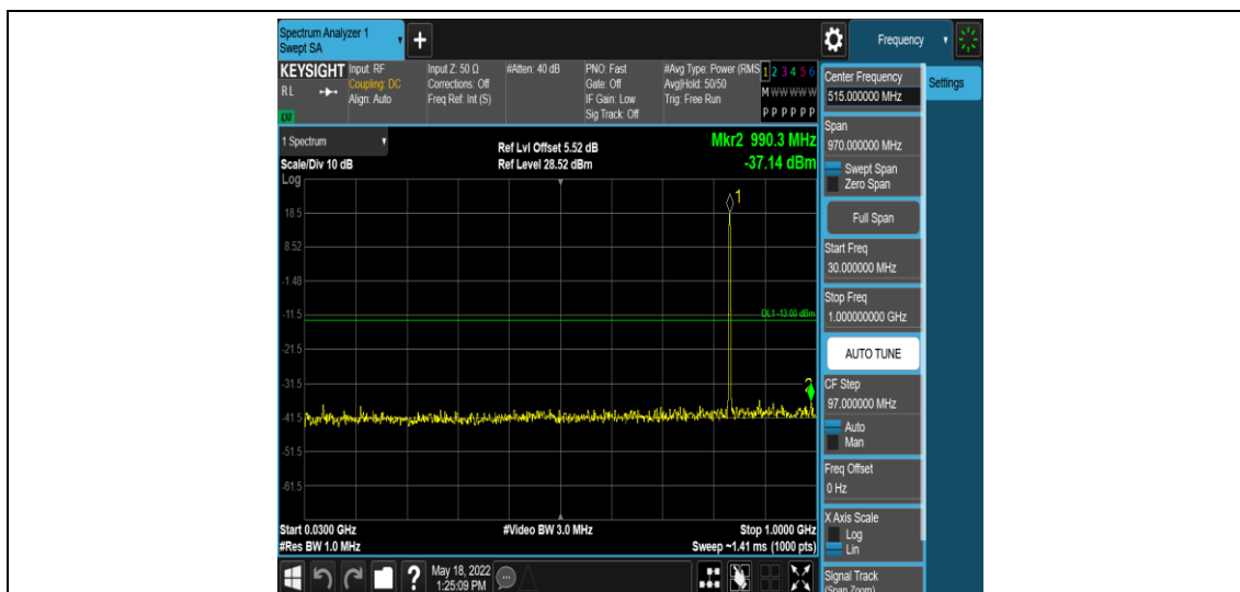
Band5-1.4MHz-QPSK-20525-1RB#0-Range3:30~1000MHz
