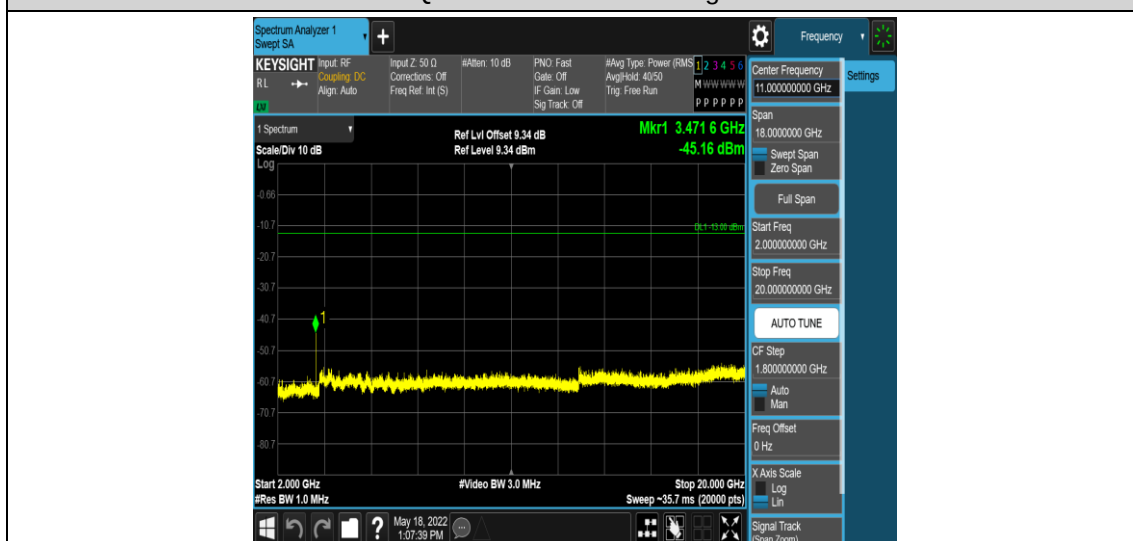
Band4-20MHz-16QAM-20300-1RB#0-Range5:2000~20000MHz
