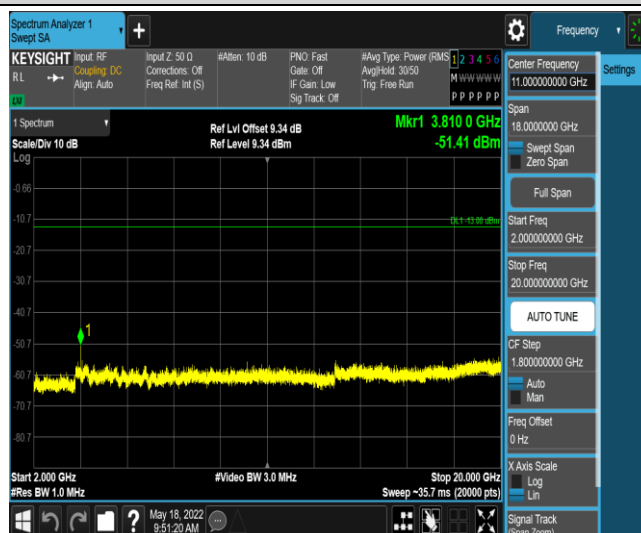
Band2-5MHz-16QAM-19175-1RB#0-Range5:2000~20000MHz
