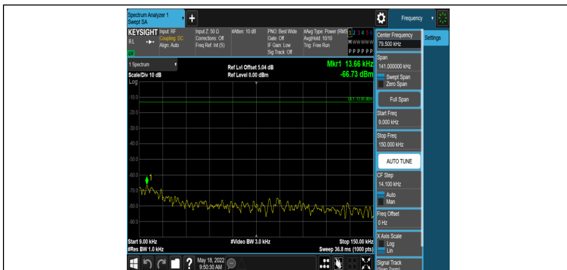
Band2-5MHz-16QAM-19175-1RB#0-Range1:0.009~0.15MHz
