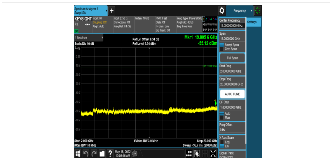
Band2-10MHz-16QAM-18650-1RB#0-Range5:2000~20000MHz
