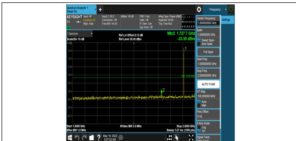
Band2-1.4MHz-16QAM-19193-1RB#0-Range4:1000~2000MHz
