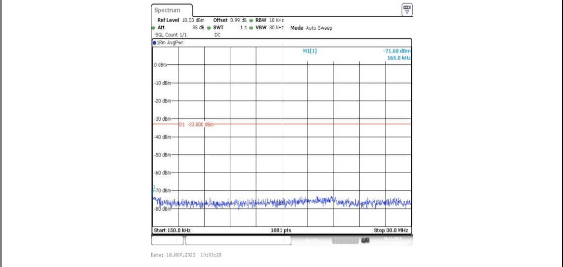
Band4-1312-0.15-30MHz-PASS
