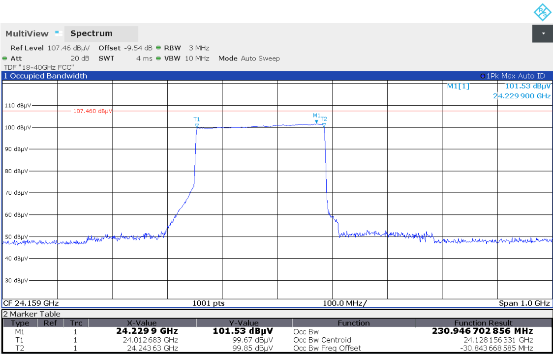
Plots No.11: 99% Occupied Bandwidth, Horizontal / Vertical Polarization
