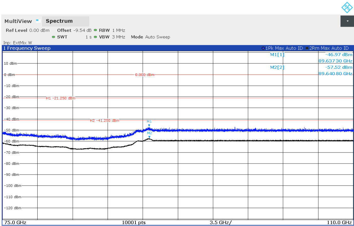
Plots No. 10: 75 GHz to 110 GHz, Horizontal / Vertical Polarization
