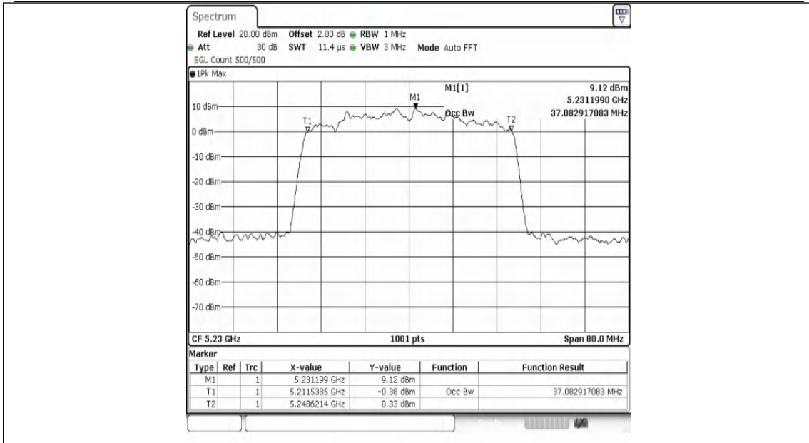
11AX40SISO-Ant1-5230
